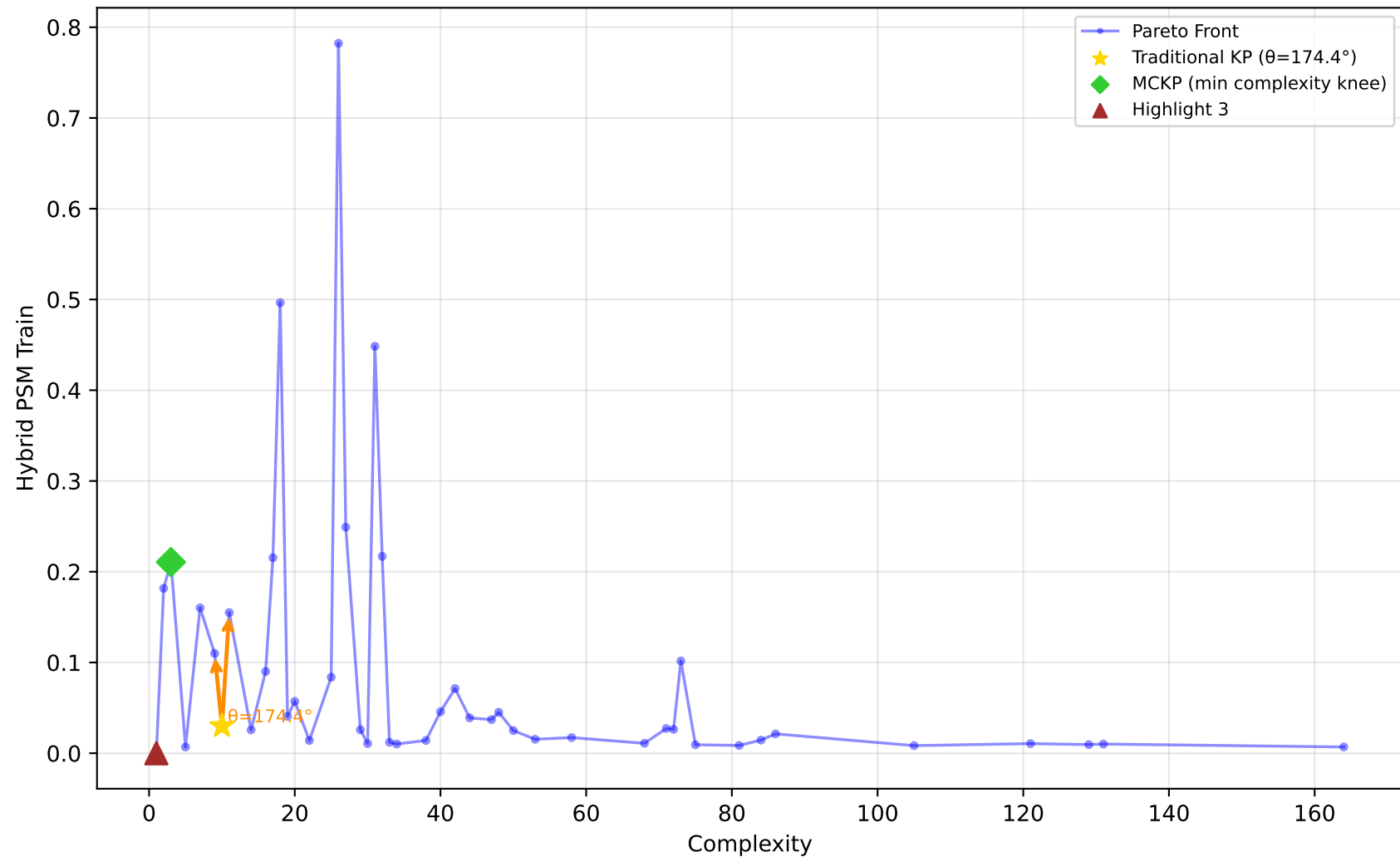
584_fri_c4_500_25 - Run 1 - SVP - Hybrid PSM Train \lambda_1=0.10, \lambda_2=0.40, \lambda_3=0.00 | Difficulty: 1.00 | Method: hmr
