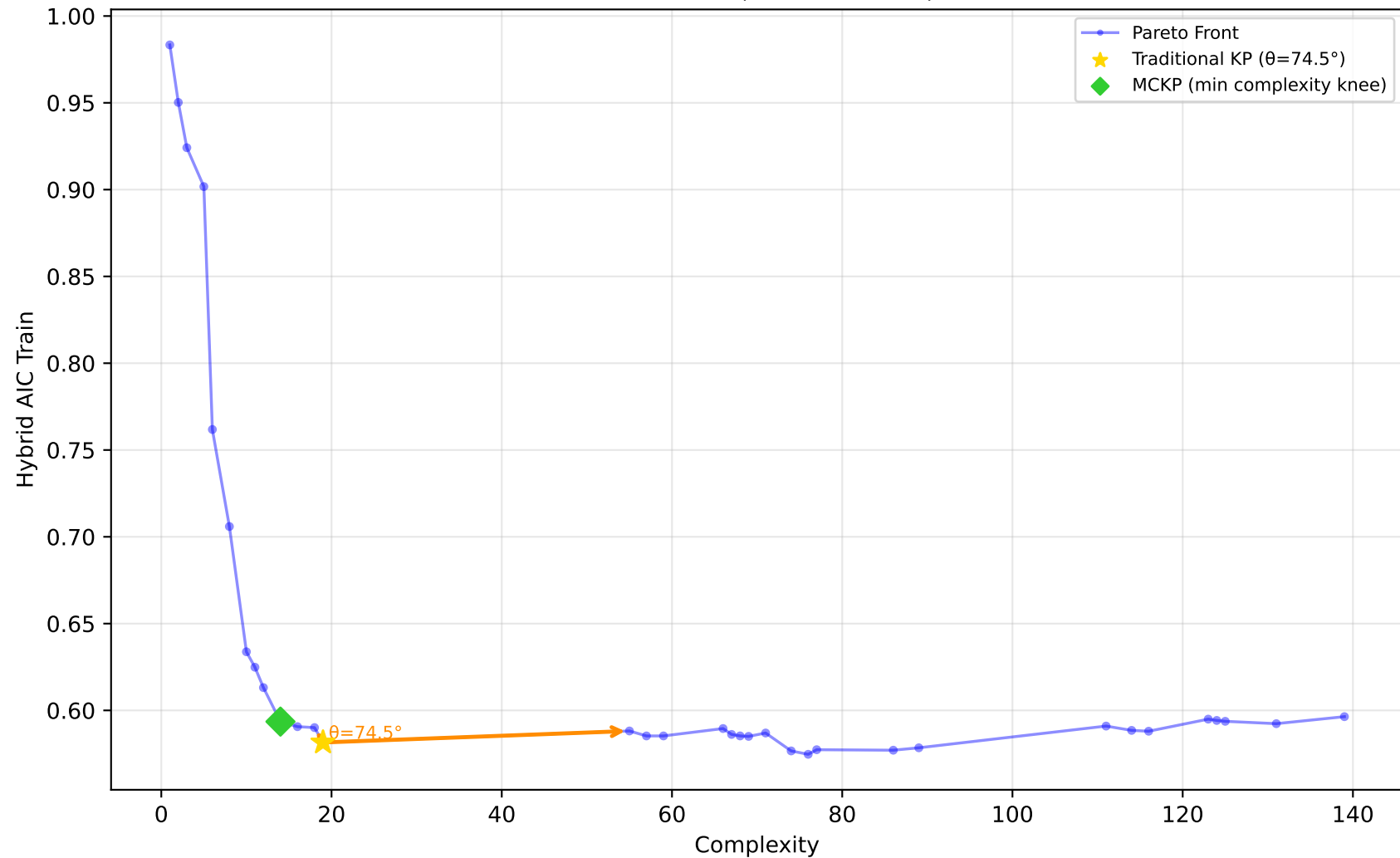
584_fri_c4_500_25 - Run 20 - MVP - Hybrid AIC Train \lambda_1=0.00, \lambda_2=0.00, \lambda_3=0.00 | Difficulty: 1.00 | Method: hmr
