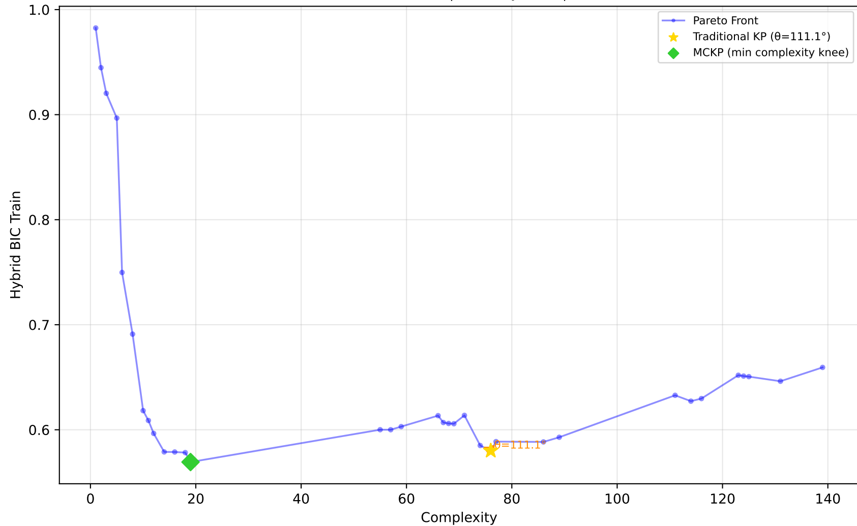
584_fri_c4_500_25 - Run 20 - MVP - Hybrid BIC Train \lambda_1=0.00, \lambda_2=0.00, \lambda_3=0.00 | Difficulty: 1.00 | Method: hmr
