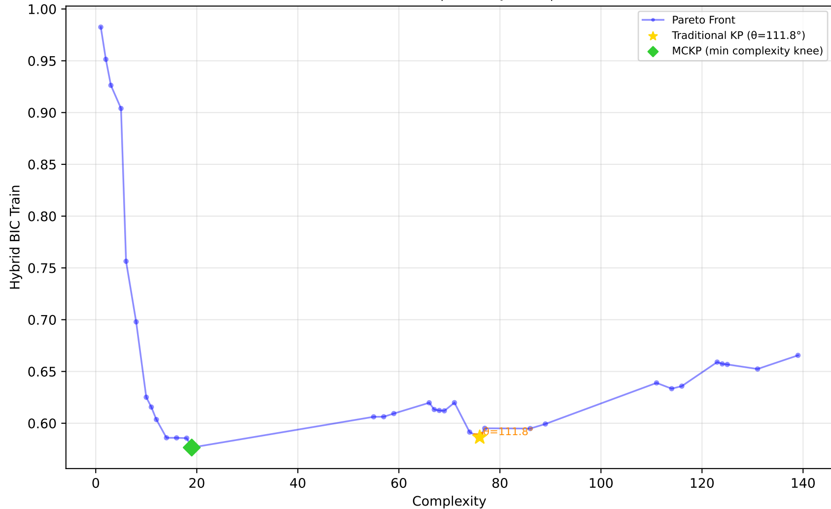
584_fri_c4_500_25 - Run 20 - MVP - Hybrid BIC Train \lambda_1=0.10, \lambda_2=0.00, \lambda_3=0.00 | Difficulty: 1.00 | Method: hmr
