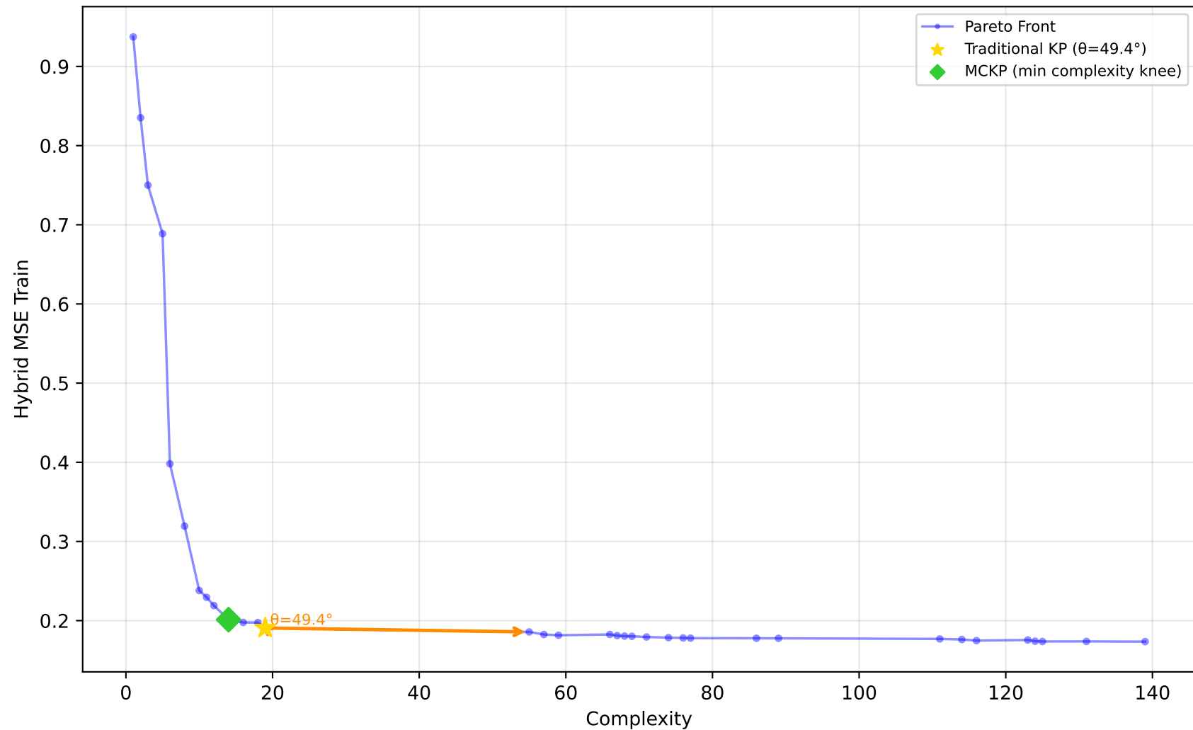
584_fri_c4_500_25 - Run 20 - MVP - Hybrid MSE Train \lambda_1=0.10, \bar{\lambda}_2=0.00, \bar{\lambda}_3=0.00 | Difficulty: 1.00 | Method: hmr
