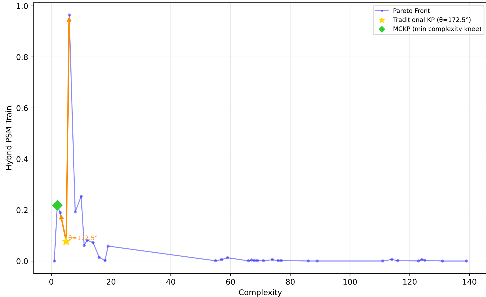
584_fri_c4_500_25 - Run 20 - MVP - Hybrid PSM Train \lambda_1=0.00, \bar{\lambda}_2=0.00, \bar{\lambda}_3=0.00 | Difficulty: 1.00 | Method: hmr
