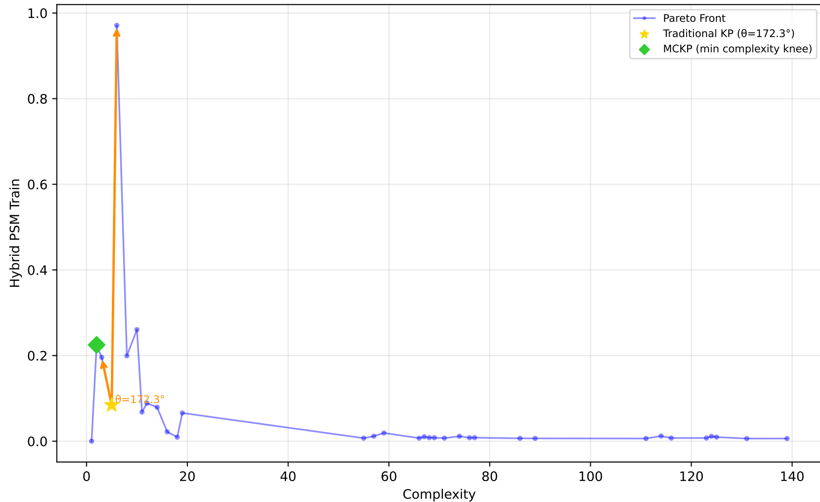
584_fri_c4_500_25 - Run 20 - MVP - Hybrid PSM Train \lambda_1=0.10, \bar{\lambda}_2=0.00, \bar{\lambda}_3=0.00 | Difficulty: 1.00 | Method: hmr
