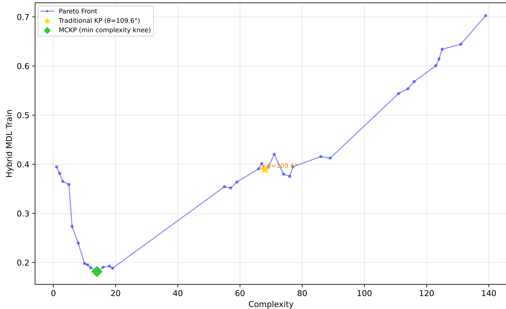
584_fri_c4_500_25 - Run 20 - SVP - Hybrid MDL Train \lambda_1=0.10, \lambda_2=0.40, \lambda_3=0.00 | Difficulty: 1.00 | Method: hmr
