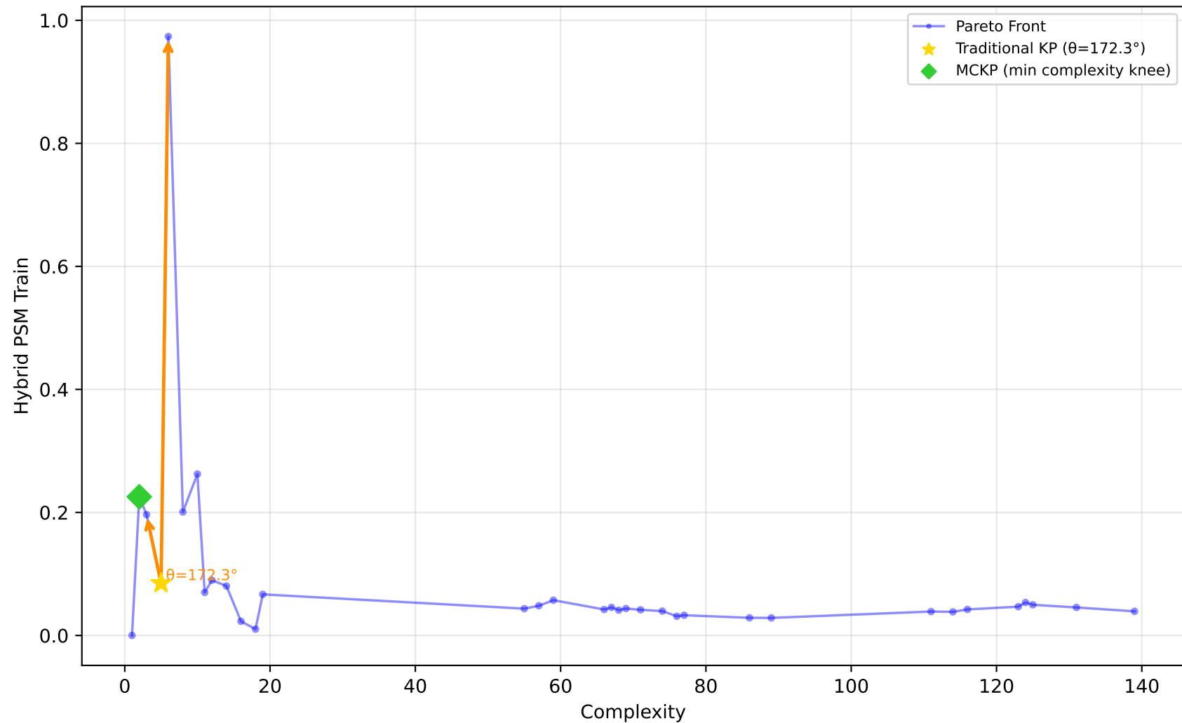
584_fri_c4_500_25 - Run 20 - SVP - Hybrid PSM Train \lambda_1=0.10, \lambda_2=0.40, \lambda_3=0.00 | Difficulty: 1.00 | Method: hmr
