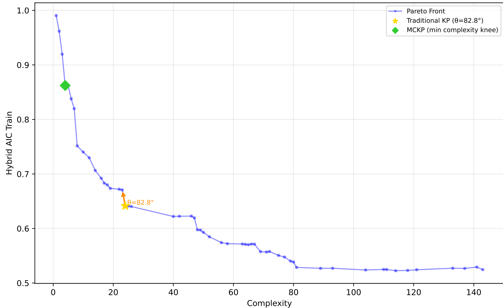
584_fri_c4_500_25 - Run 21 - MVP - Hybrid AIC Train \lambda_1=0.00, \lambda_2=0.00, \lambda_3=0.00 | Difficulty: 1.00 | Method: hmr
