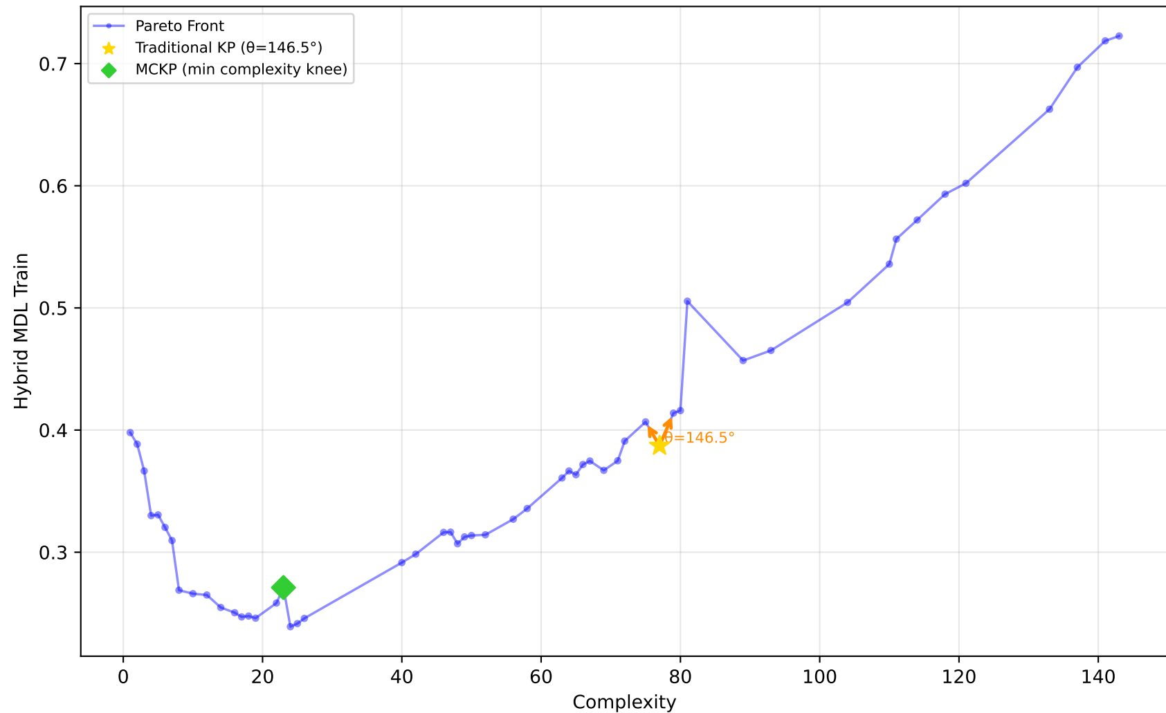
584_fri_c4_500_25 - Run 21 - MVP - Hybrid MDL Train \lambda_1=0.10, \bar{\lambda}_2=0.00, \bar{\lambda}_3=0.00 | Difficulty: 1.00 | Method: hmr
