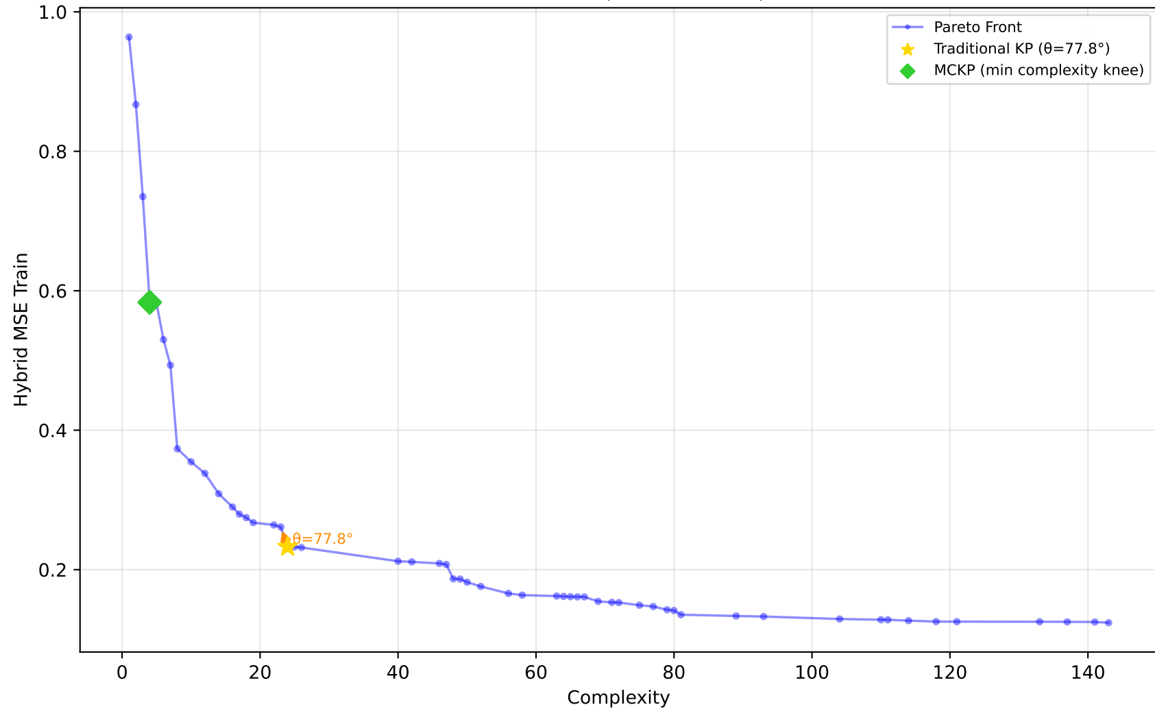
584_fri_c4_500_25 - Run 21 - MVP - Hybrid MSE Train \lambda_1=0.00, \bar{\lambda}_2=0.00, \lambda_3=0.00 | Difficulty: 1.00 | Method: hmr
