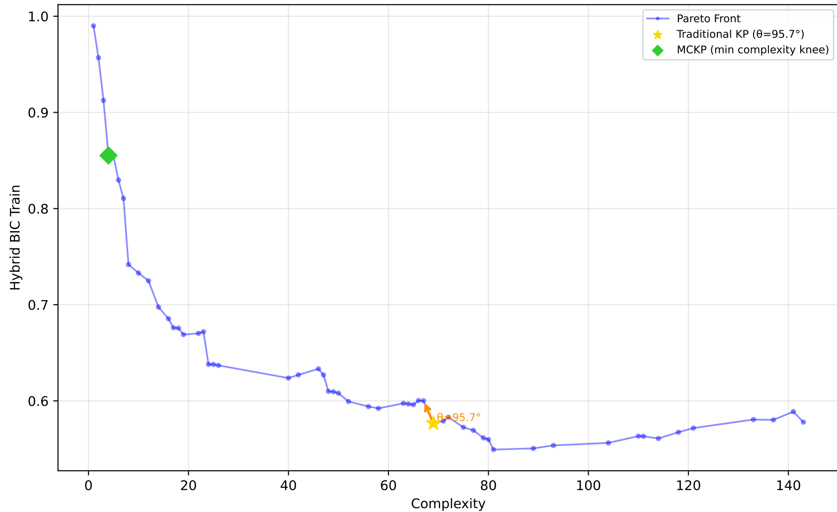
584_fri_c4_500_25 - Run 21 - SVP - Hybrid BIC Train \lambda_1=0.00, \lambda_2=0.00, \lambda_3=0.00 | Difficulty: 1.00 | Method: hmr
