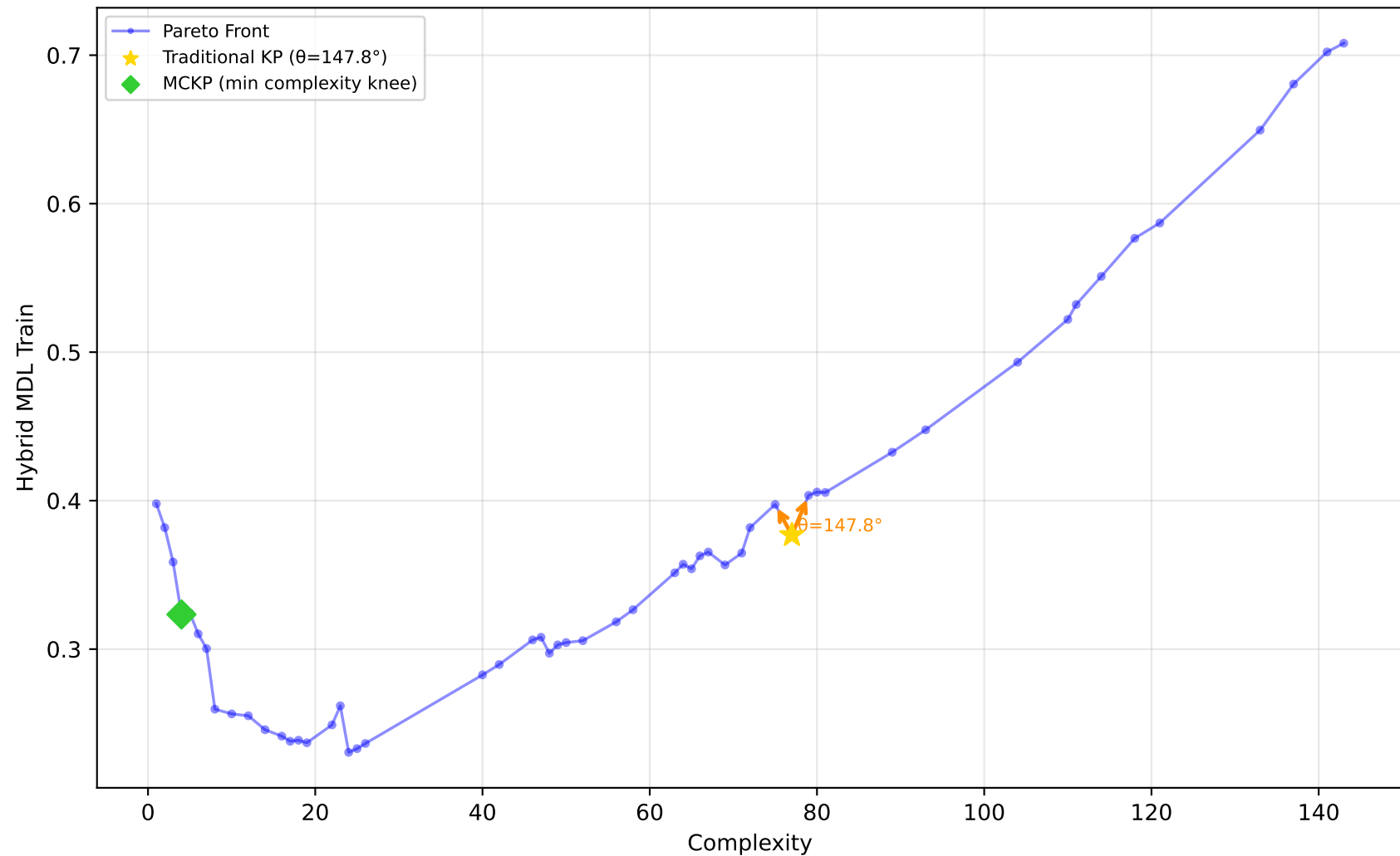
584_fri_c4_500_25 - Run 21 - SVP - Hybrid MDL Train \lambda_1=0.00, \lambda_2=0.00, \lambda_3=0.00 | Difficulty: 1.00 | Method: hmr
