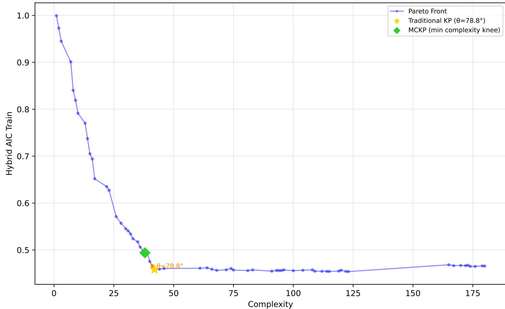
584_fri_c4_500_25 - Run 22 - MVP - Hybrid AIC Train \lambda_1=0.00, \lambda_2=0.00, \lambda_3=0.00 | Difficulty: 1.00 | Method: hmr
