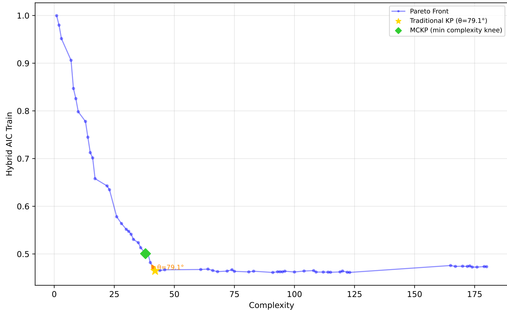
584_fri_c4_500_25 - Run 22 - MVP - Hybrid AIC Train \lambda_1=0.10, \lambda_2=0.00, \lambda_3=0.00 | Difficulty: 1.00 | Method: hmr
