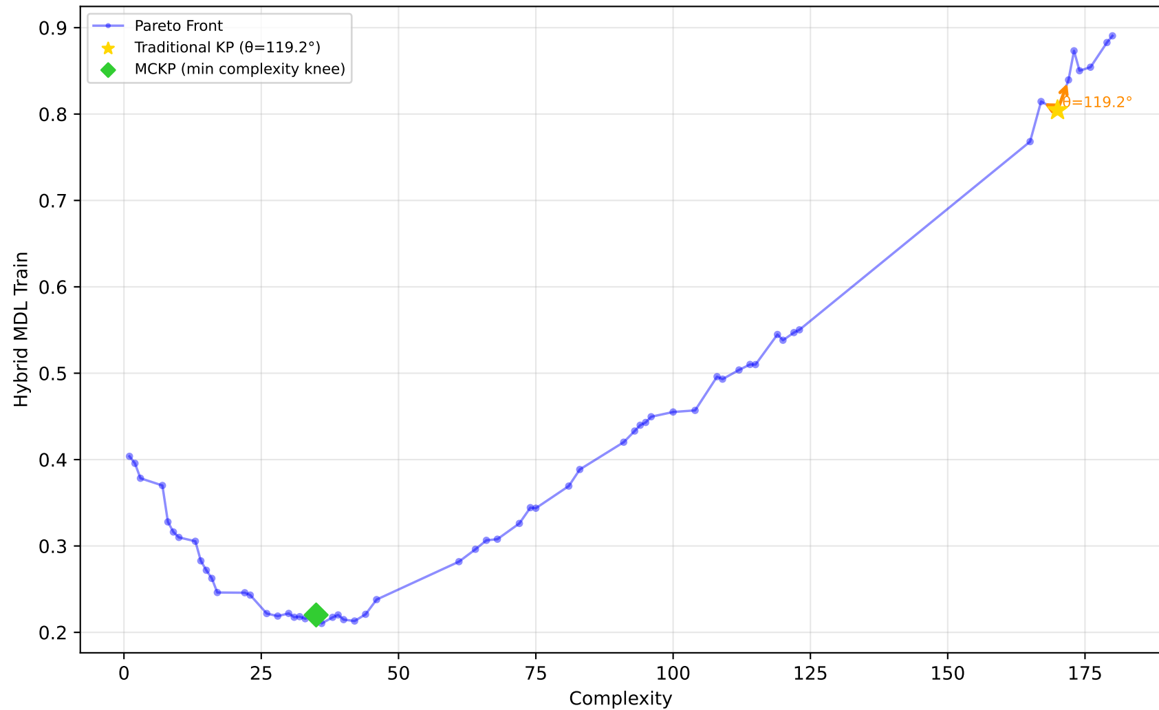
584_fri_c4_500_25 - Run 22 - MVP - Hybrid MDL Train \lambda_1=0.10, \bar{\lambda}_2=0.00, \bar{\lambda}_3=0.00 | Difficulty: 1.00 | Method: hmr
