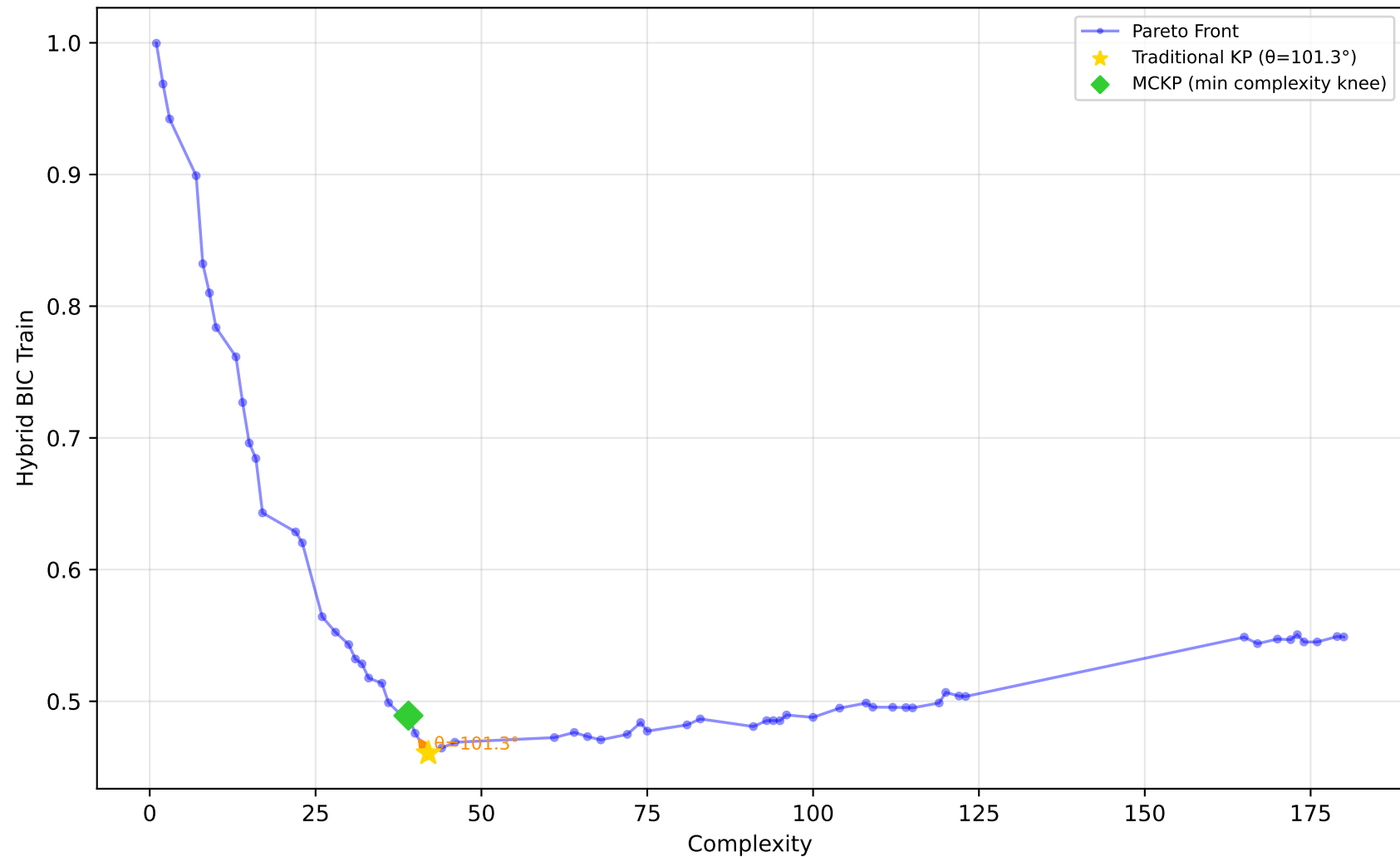
584_fri_c4_500_25 - Run 22 - SVP - Hybrid BIC Train \lambda_1=0.00, \lambda_2=0.00, \lambda_3=0.00 | Difficulty: 1.00 | Method: hmr
