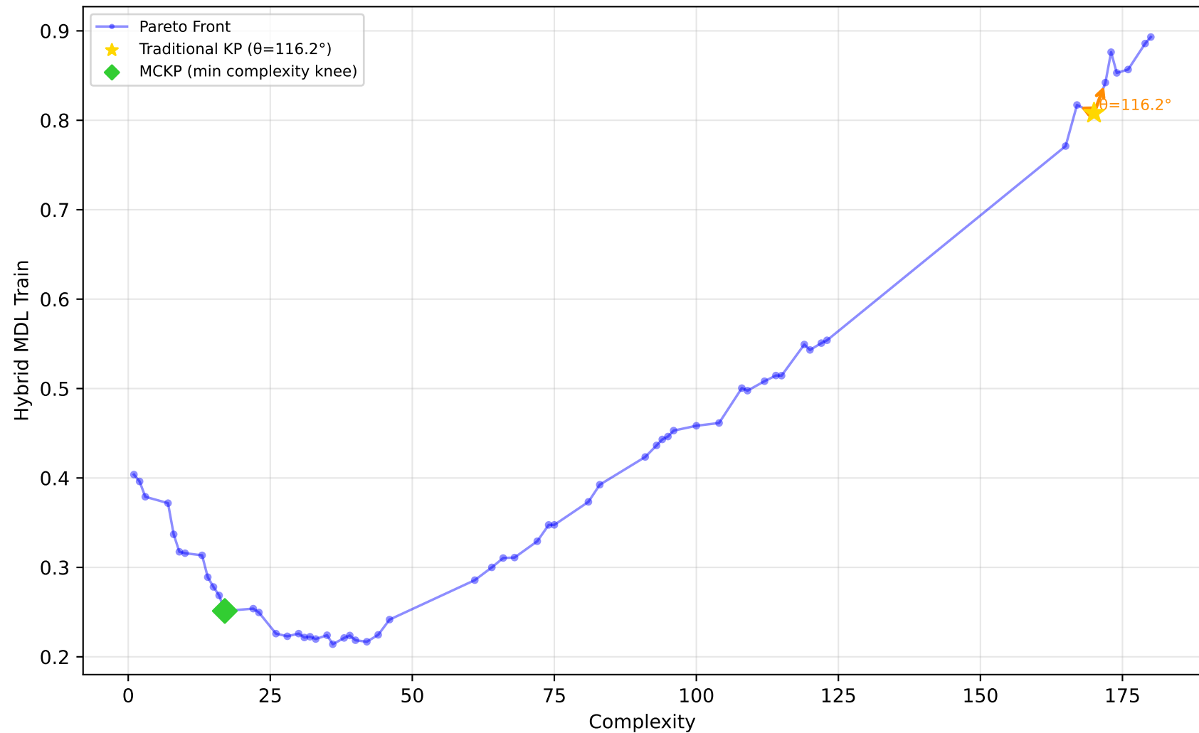
584_fri_c4_500_25 - Run 22 - SVP - Hybrid MDL Train \lambda_1=0.10, \lambda_2=0.40, \lambda_3=0.00 | Difficulty: 1.00 | Method: hmr
