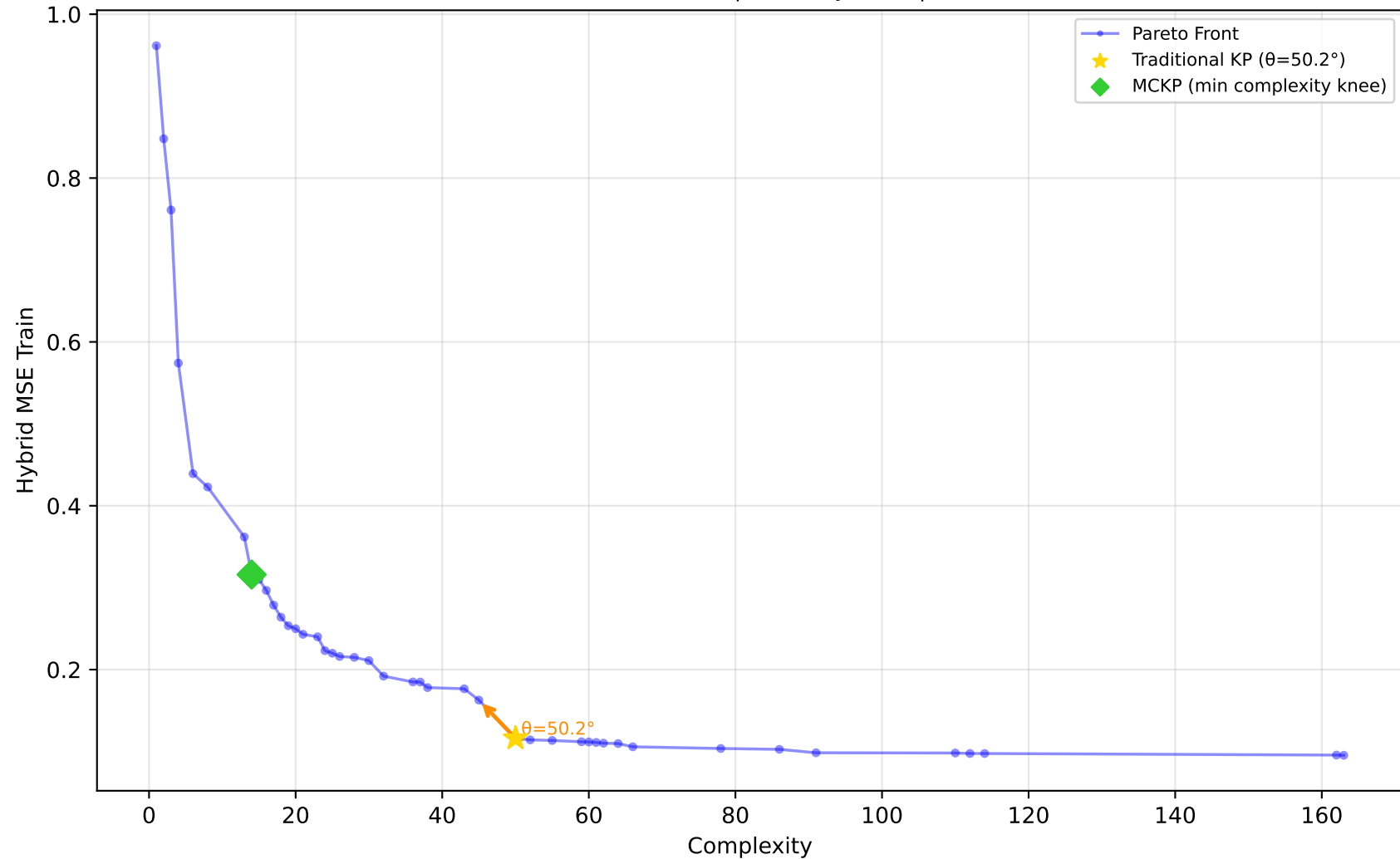
584_fri_c4_500_25 - Run 23 - MVP - Hybrid MSE Train \lambda_1=0.00, \bar{\lambda}_2=0.00, \bar{\lambda}_3=0.00 | Difficulty: 1.00 | Method: hmr
