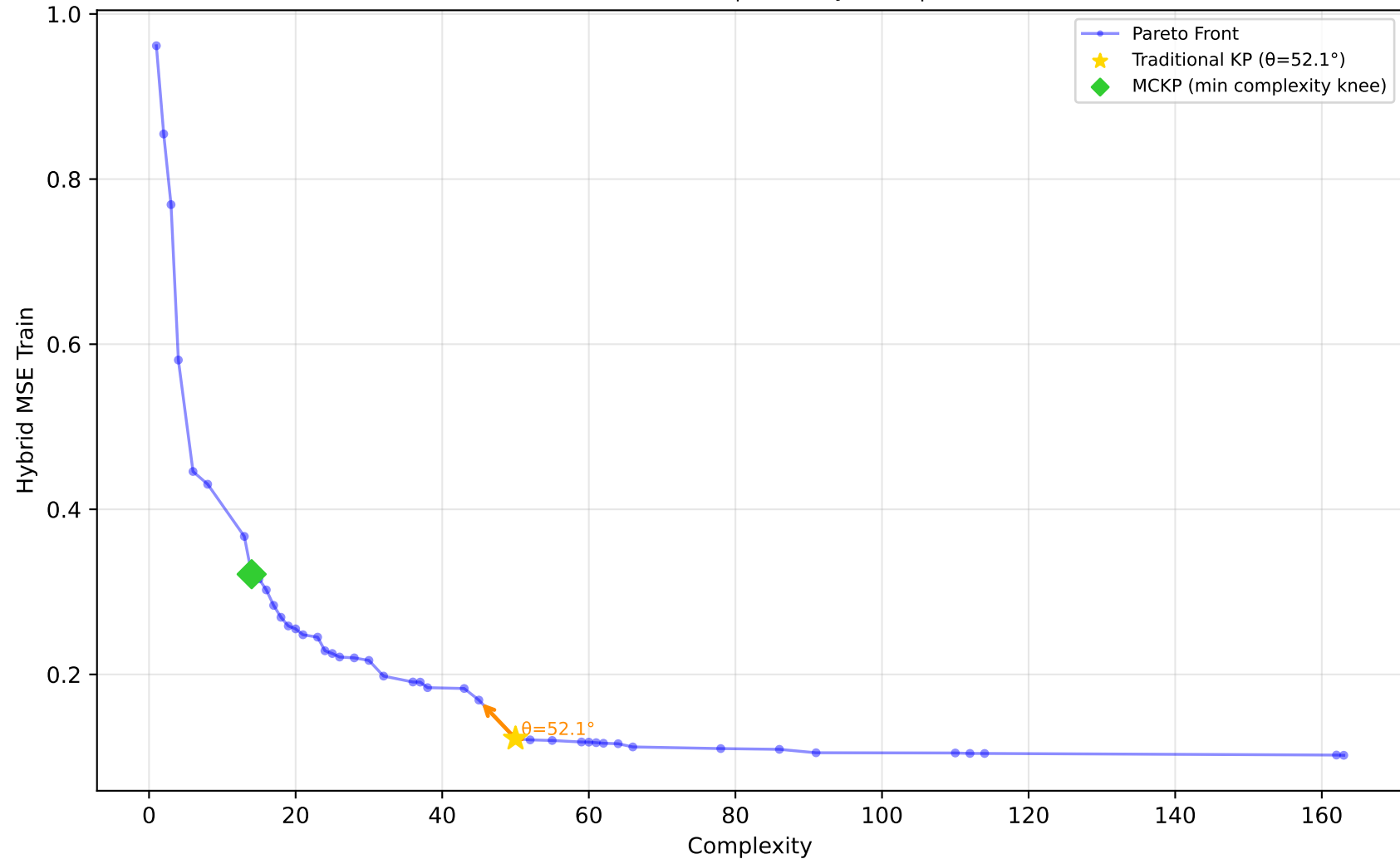
584_fri_c4_500_25 - Run 23 - MVP - Hybrid MSE Train \lambda_1=0.10, \bar{\lambda}_2=0.00, \bar{\lambda}_3=0.00 | Difficulty: 1.00 | Method: hmr
