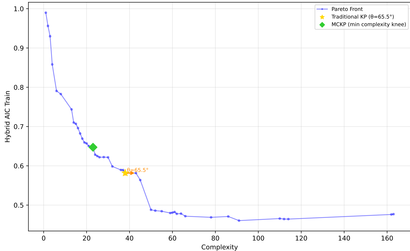
584_fri_c4_500_25 - Run 23 - SVP - Hybrid AIC Train \lambda_1=0.00, \lambda_2=0.00, \lambda_3=0.00 | Difficulty: 1.00 | Method: hmr
