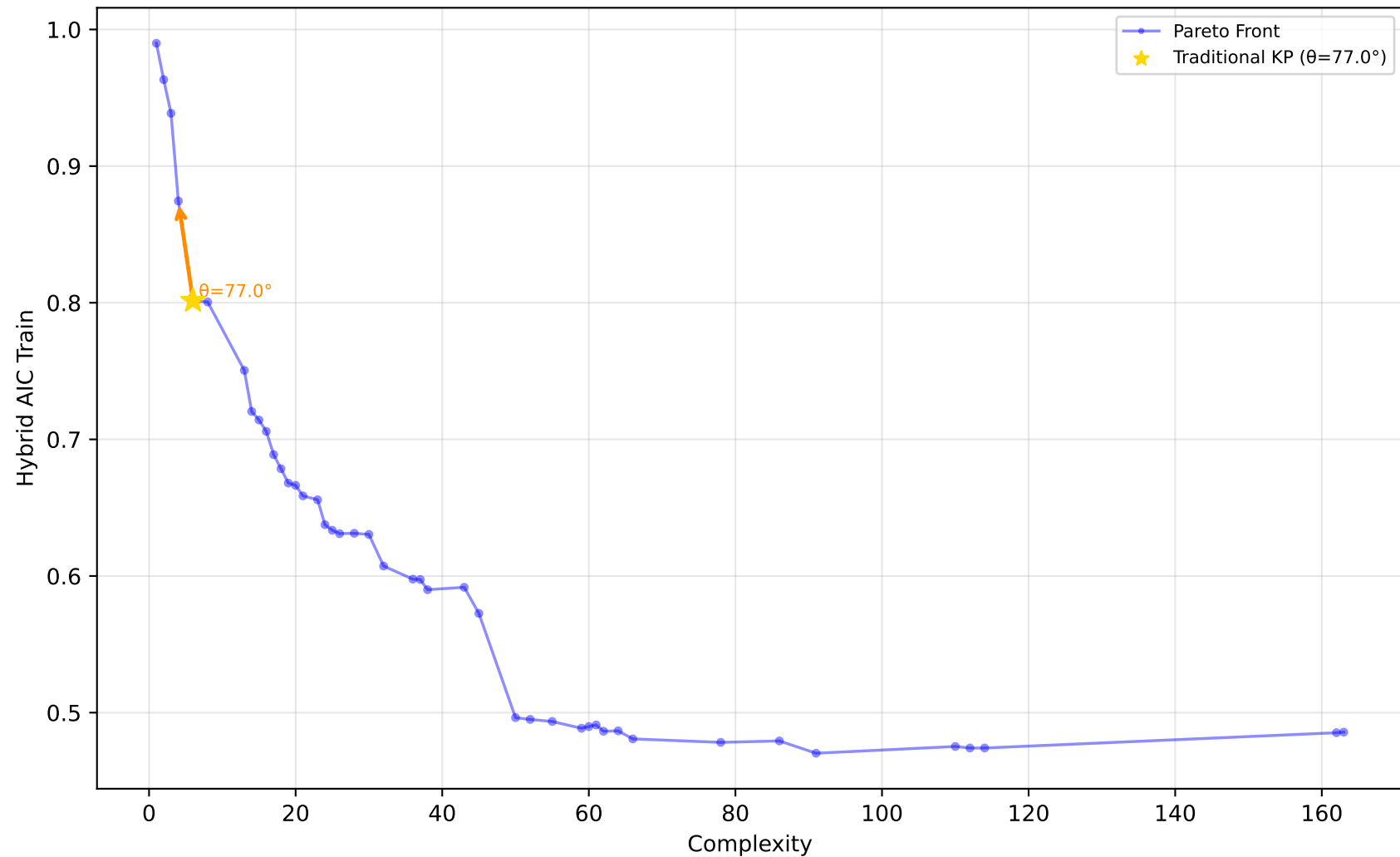
584_fri_c4_500_25 - Run 23 - SVP - Hybrid AIC Train \lambda_1=0.10, \lambda_2=0.40, \lambda_3=0.00 | Difficulty: 1.00 | Method: hmr
