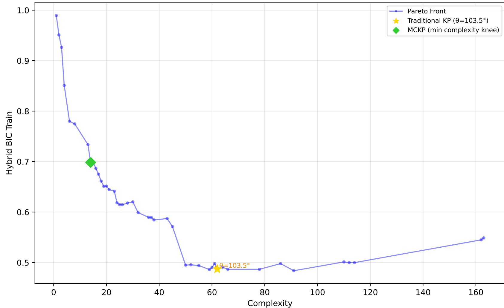
584_fri_c4_500_25 - Run 23 - SVP - Hybrid BIC Train \lambda_1=0.00 , \lambda_2=0.00 , \lambda_3=0.00 | Difficulty: 1.00 | Method: hmr
