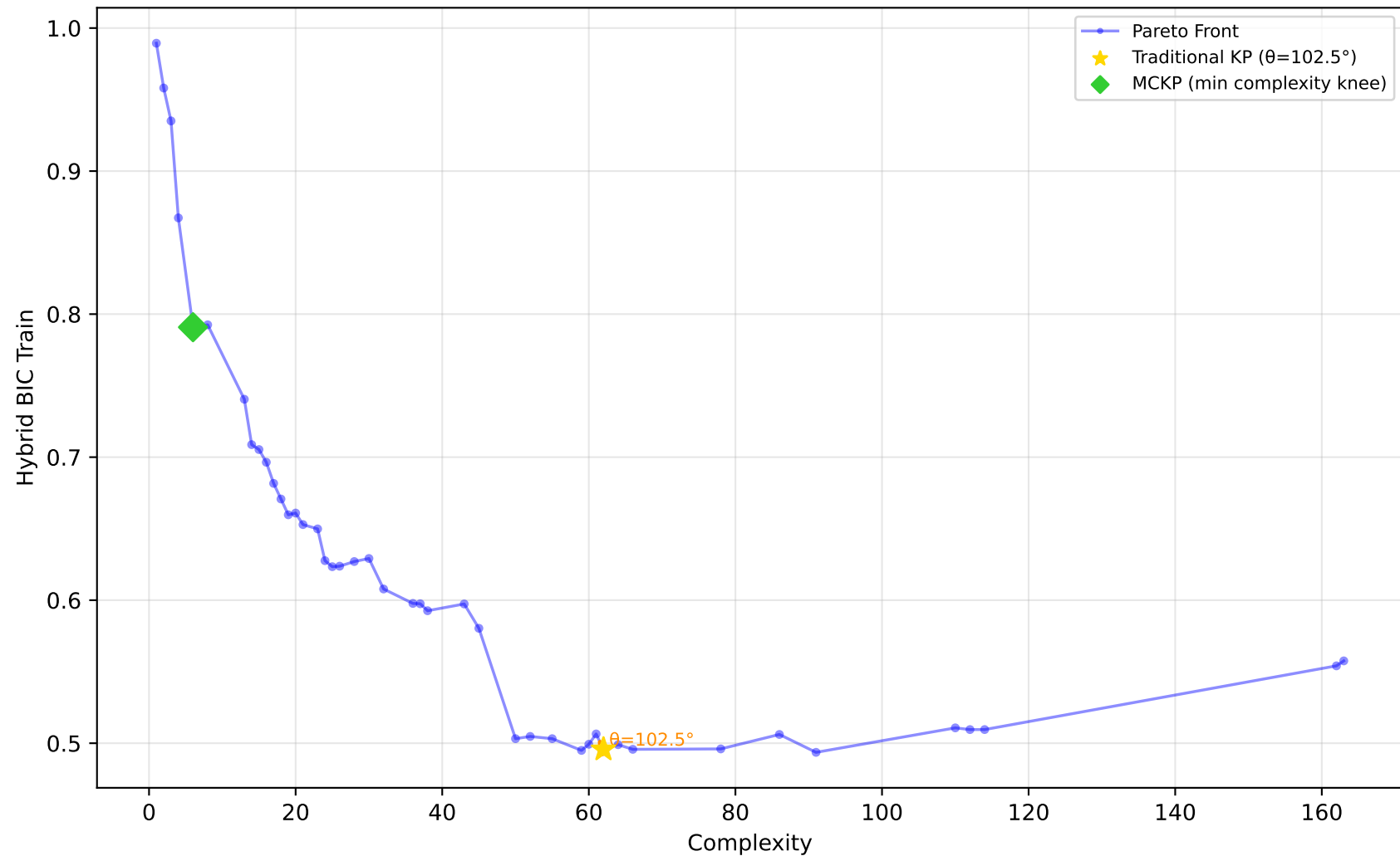
584_fri_c4_500_25 - Run 23 - SVP - Hybrid BIC Train \lambda_1=0.10 , \lambda_2=0.40 , \lambda_3=0.00 | Difficulty: 1.00 | Method: hmr
