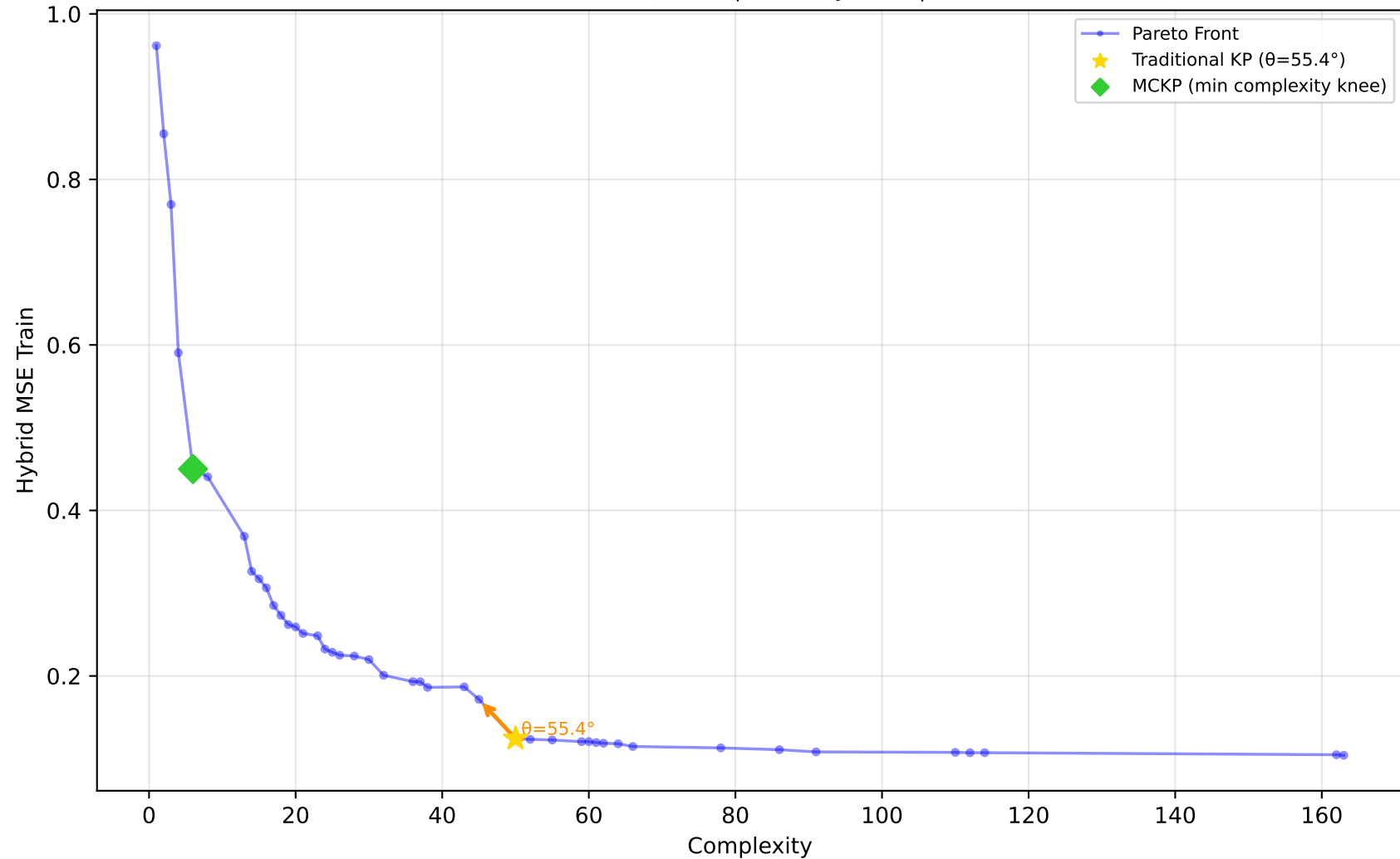
584_fri_c4_500_25 - Run 23 - SVP - Hybrid MSE Train \lambda_1=0.10, \lambda_2=0.40, \lambda_3=0.00 | Difficulty: 1.00 | Method: hmr
