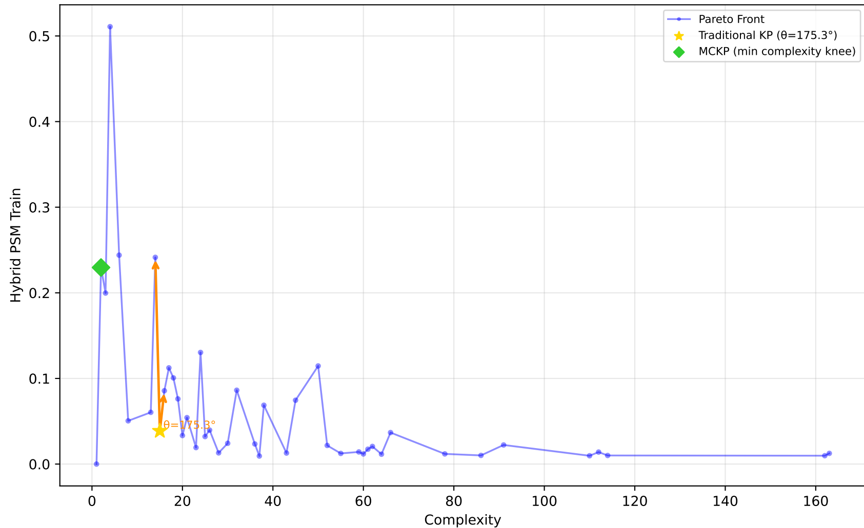
584_fri_c4_500_25 - Run 23 - SVP - Hybrid PSM Train \lambda_1=0.10, \lambda_2=0.40, \lambda_3=0.00 | Difficulty: 1.00 | Method: hmr
