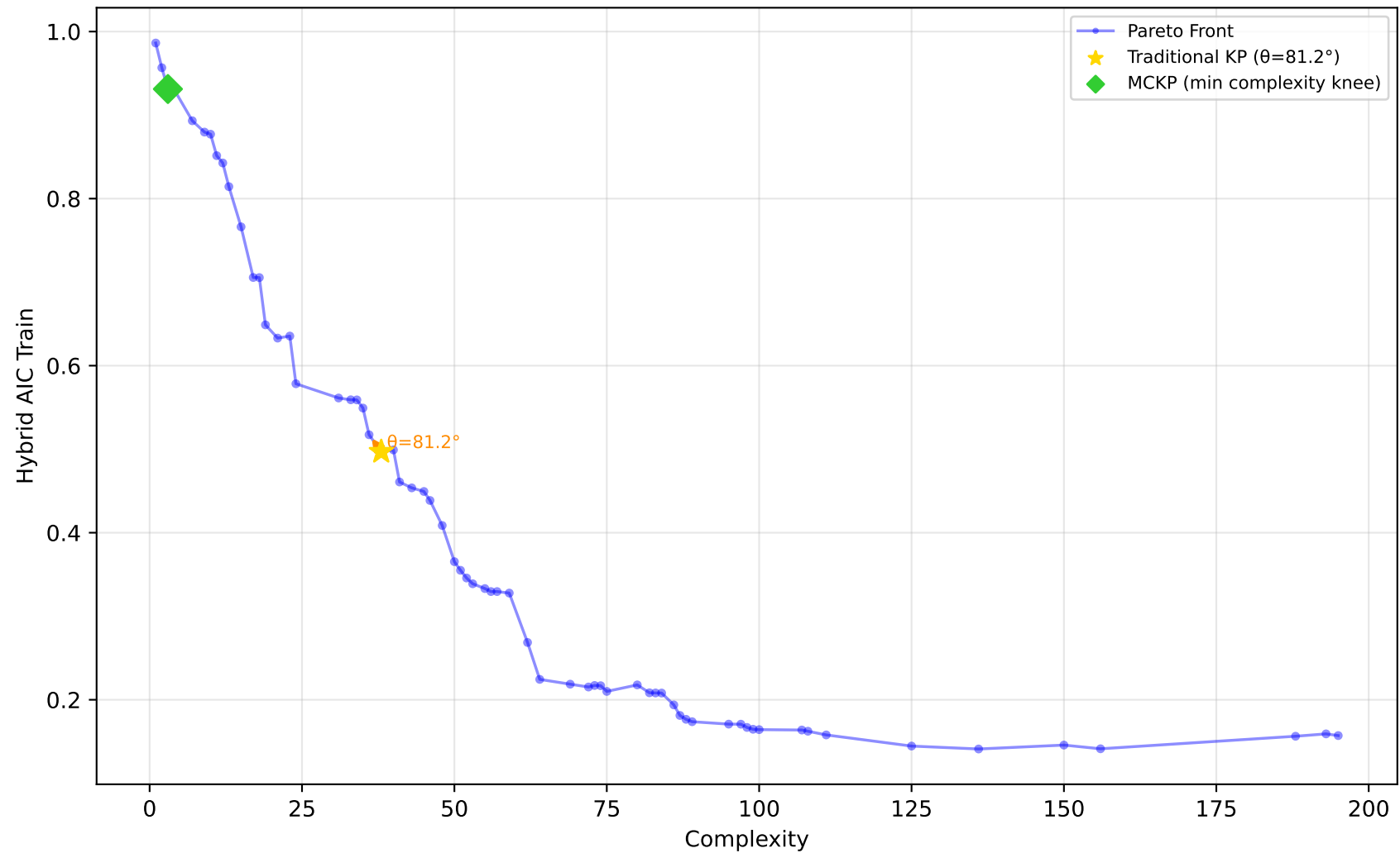
584_fri_c4_500_25 - Run 24 - MVP - Hybrid AIC Train \lambda_1=0.10, \lambda_2=0.00, \lambda_3=0.00 | Difficulty: 1.00 | Method: hmr
