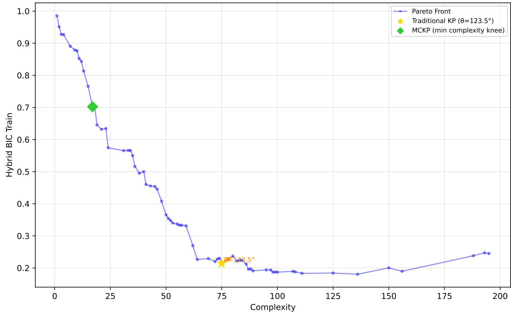
584_fri_c4_500_25 - Run 24 - MVP - Hybrid BIC Train \lambda_1=0.10, \lambda_2=0.00, \lambda_3=0.00 | Difficulty: 1.00 | Method: hmr
