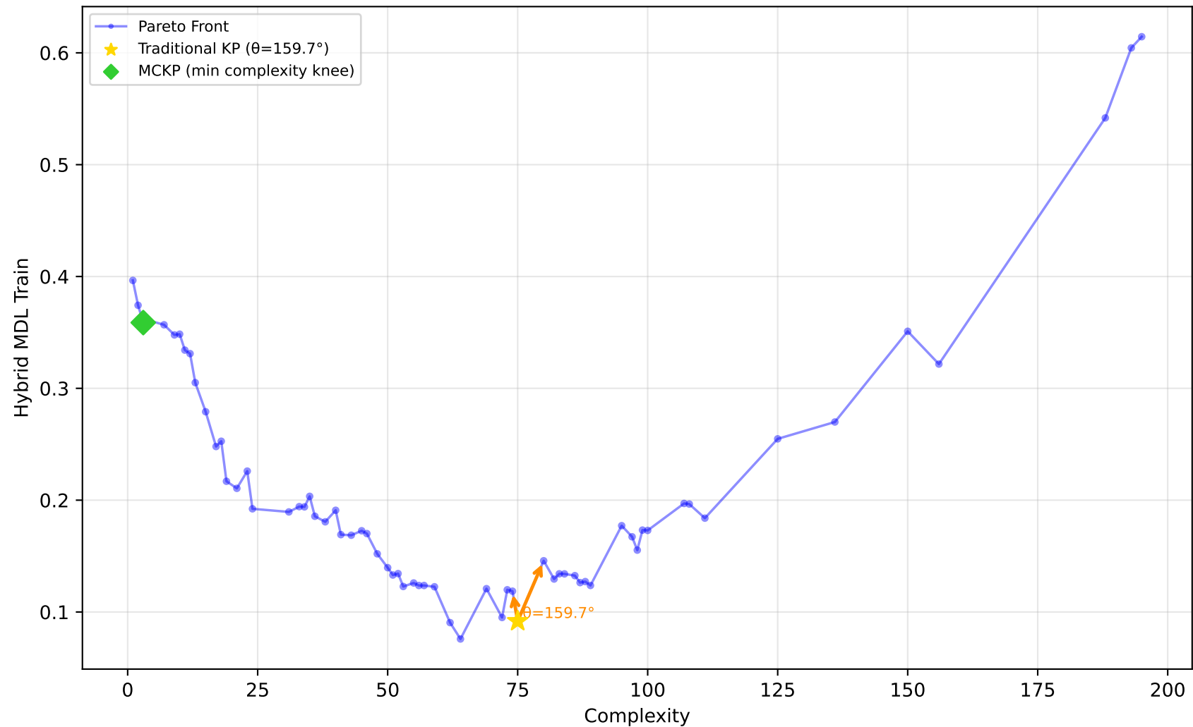
584_fri_c4_500_25 - Run 24 - MVP - Hybrid MDL Train \lambda_1=0.00, \bar{\lambda}_2=0.00, \bar{\lambda}_3=0.00 | Difficulty: 1.00 | Method: hmr
