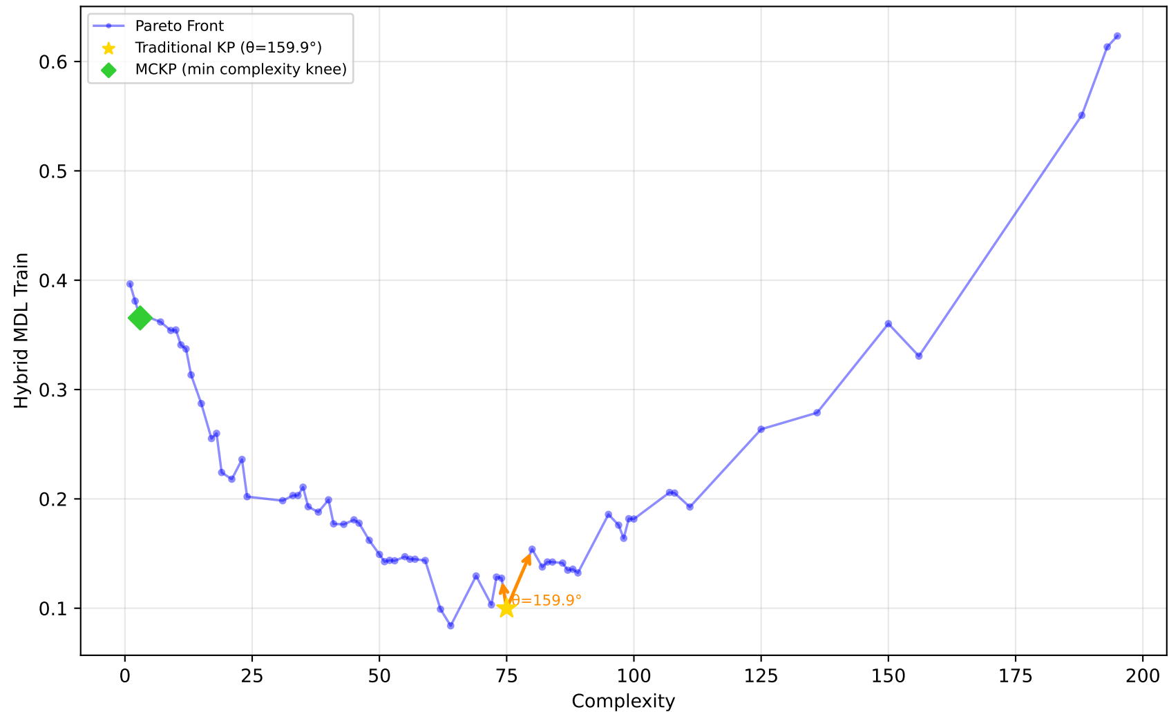
584_fri_c4_500_25 - Run 24 - MVP - Hybrid MDL Train \lambda_1=0.10, \bar{\lambda}_2=0.00, \bar{\lambda}_3=0.00 | Difficulty: 1.00 | Method: hmr
