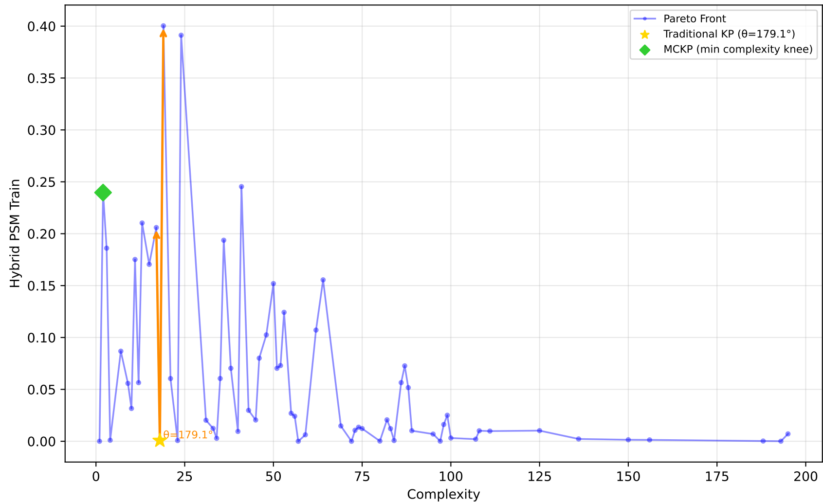
584_fri_c4_500_25 - Run 24 - MVP - Hybrid PSM Train \lambda_1=0.00, \bar{\lambda}_2=0.00, \bar{\lambda}_3=0.00 | Difficulty: 1.00 | Method: hmr
