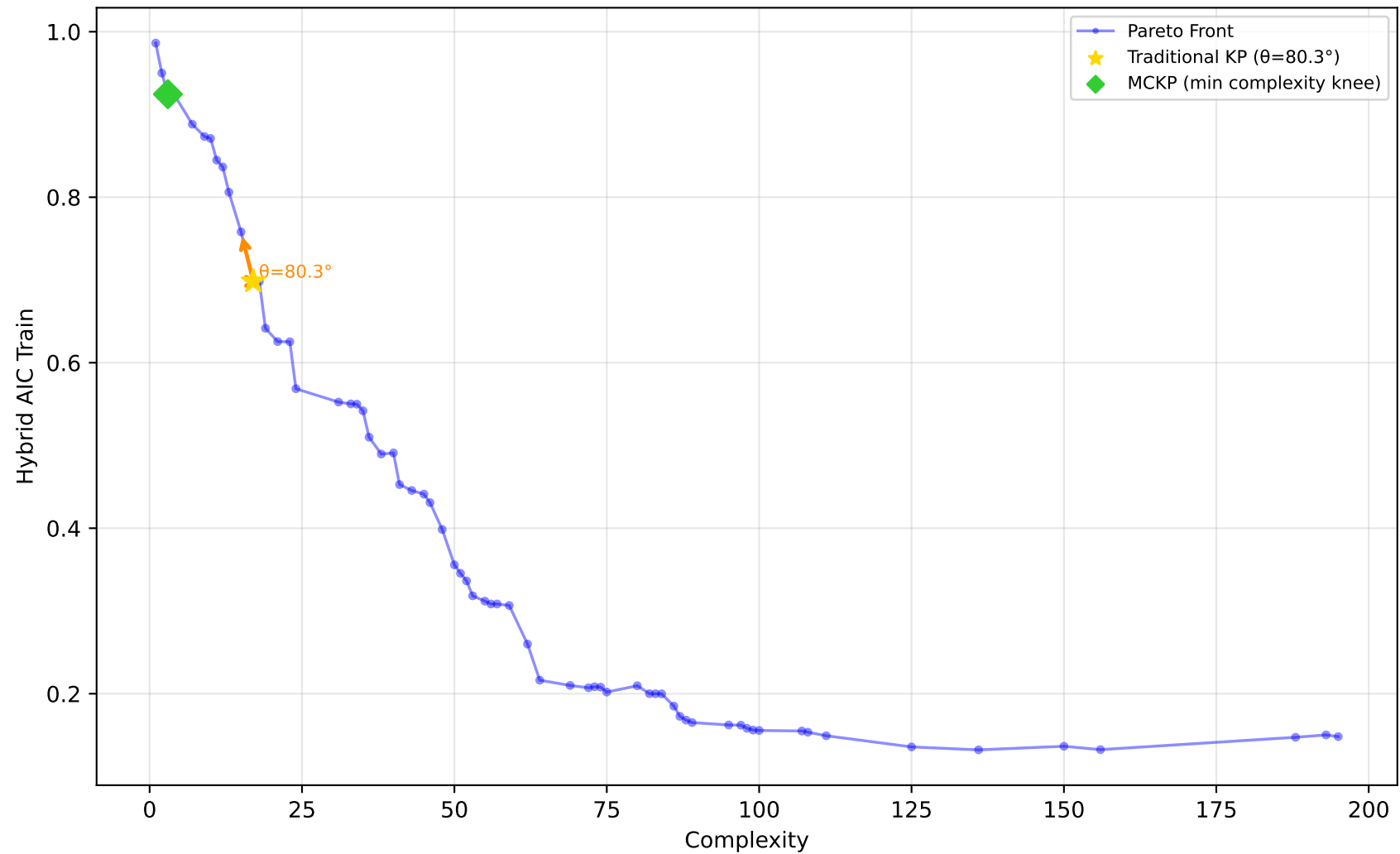
584_fri_c4_500_25 - Run 24 - SVP - Hybrid AIC Train \lambda_1=0.00, \lambda_2=0.00, \lambda_3=0.00 | Difficulty: 1.00 | Method: hmr
