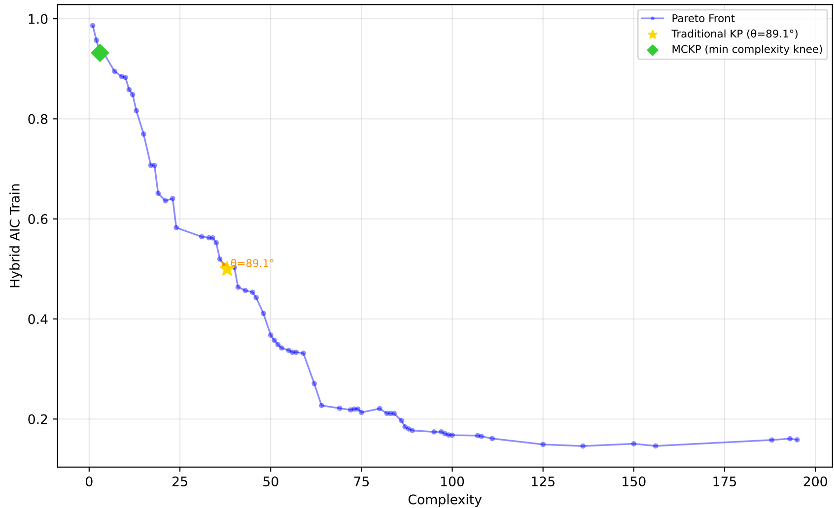
584_fri_c4_500_25 - Run 24 - SVP - Hybrid AIC Train \lambda_1=0.10, \lambda_2=0.40, \lambda_3=0.00 | Difficulty: 1.00 | Method: hmr
