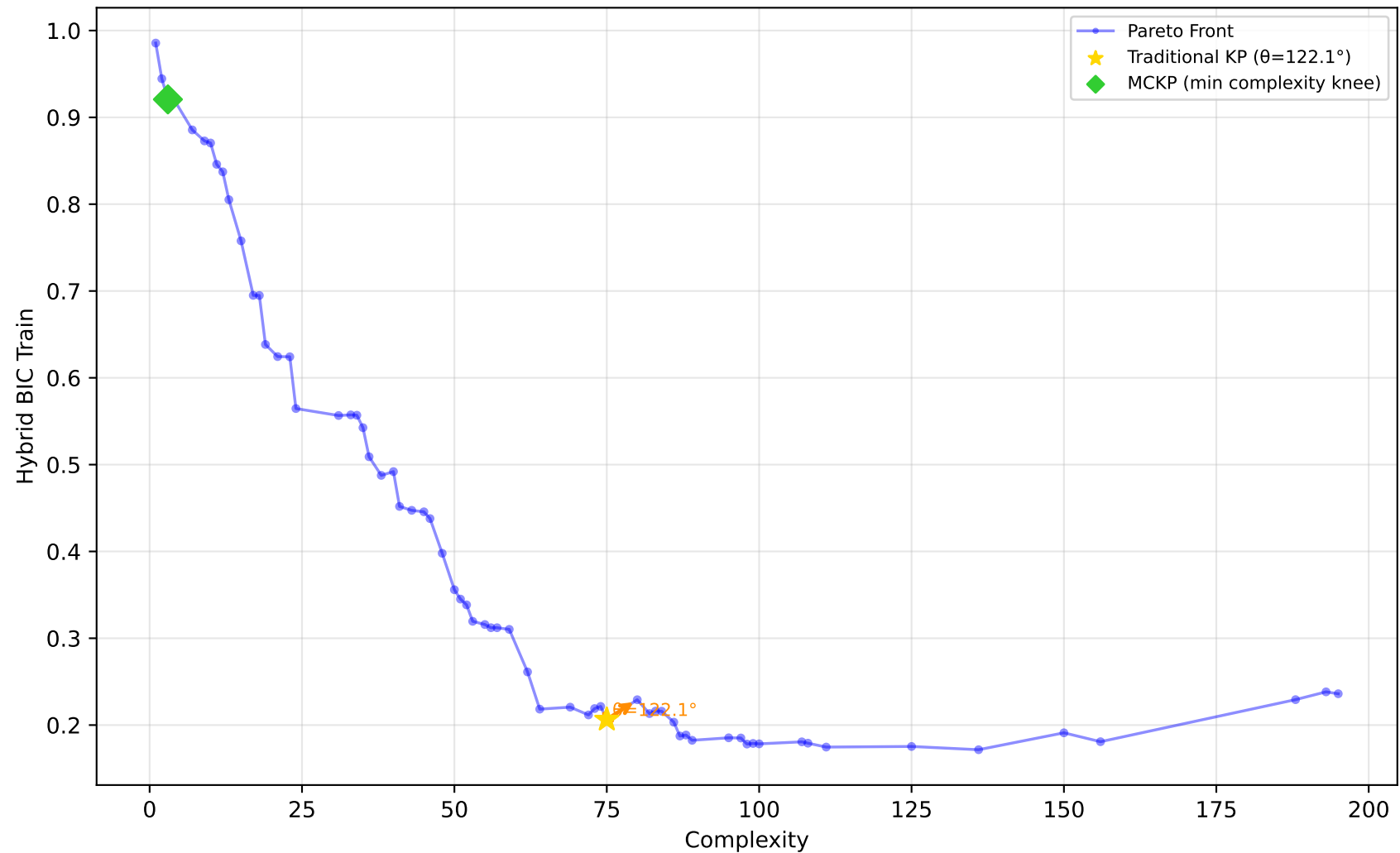
584_fri_c4_500_25 - Run 24 - SVP - Hybrid BIC Train \lambda_1=0.00, \lambda_2=0.00, \lambda_3=0.00 | Difficulty: 1.00 | Method: hmr
