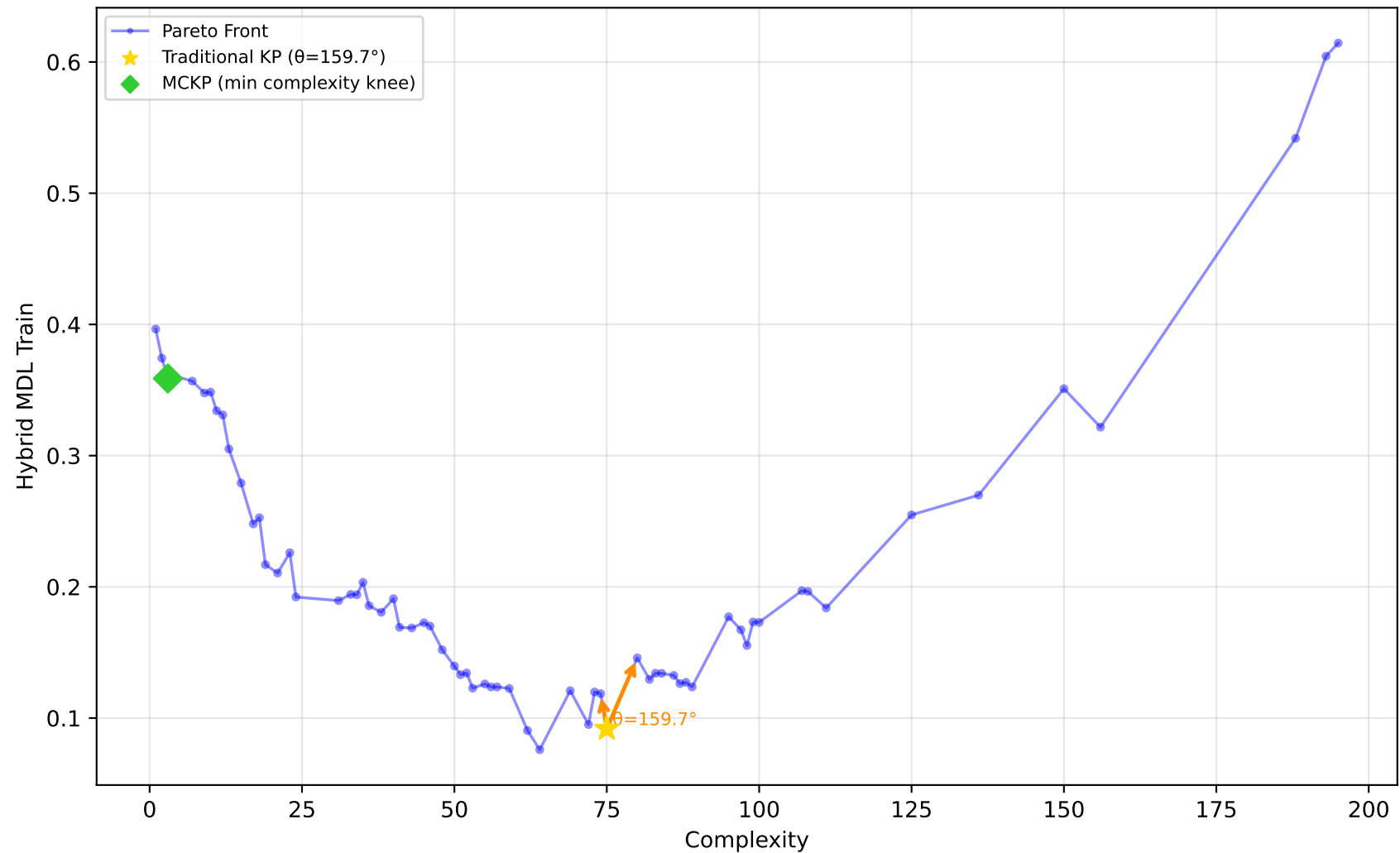
584_fri_c4_500_25 - Run 24 - SVP - Hybrid MDL Train \lambda_1=0.00, \lambda_2=0.00, \lambda_3=0.00 | Difficulty: 1.00 | Method: hmr
