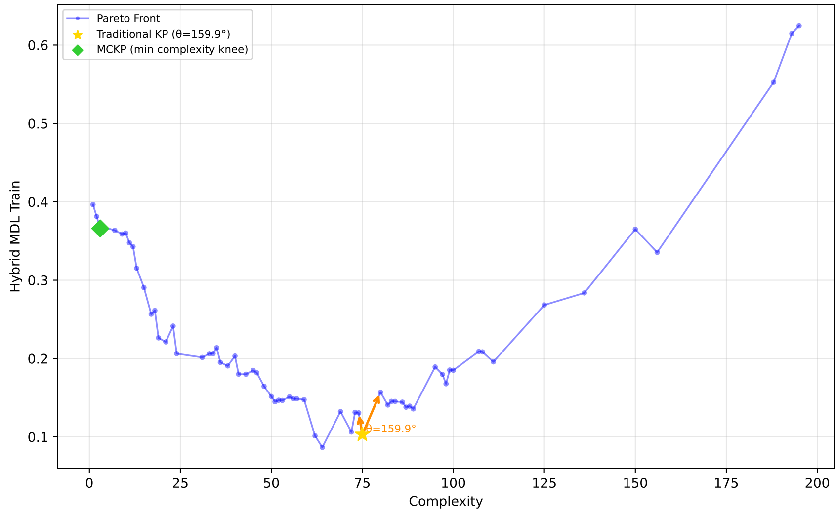
584_fri_c4_500_25 - Run 24 - SVP - Hybrid MDL Train \lambda_1=0.10, \lambda_2=0.40, \lambda_3=0.00 | Difficulty: 1.00 | Method: hmr
