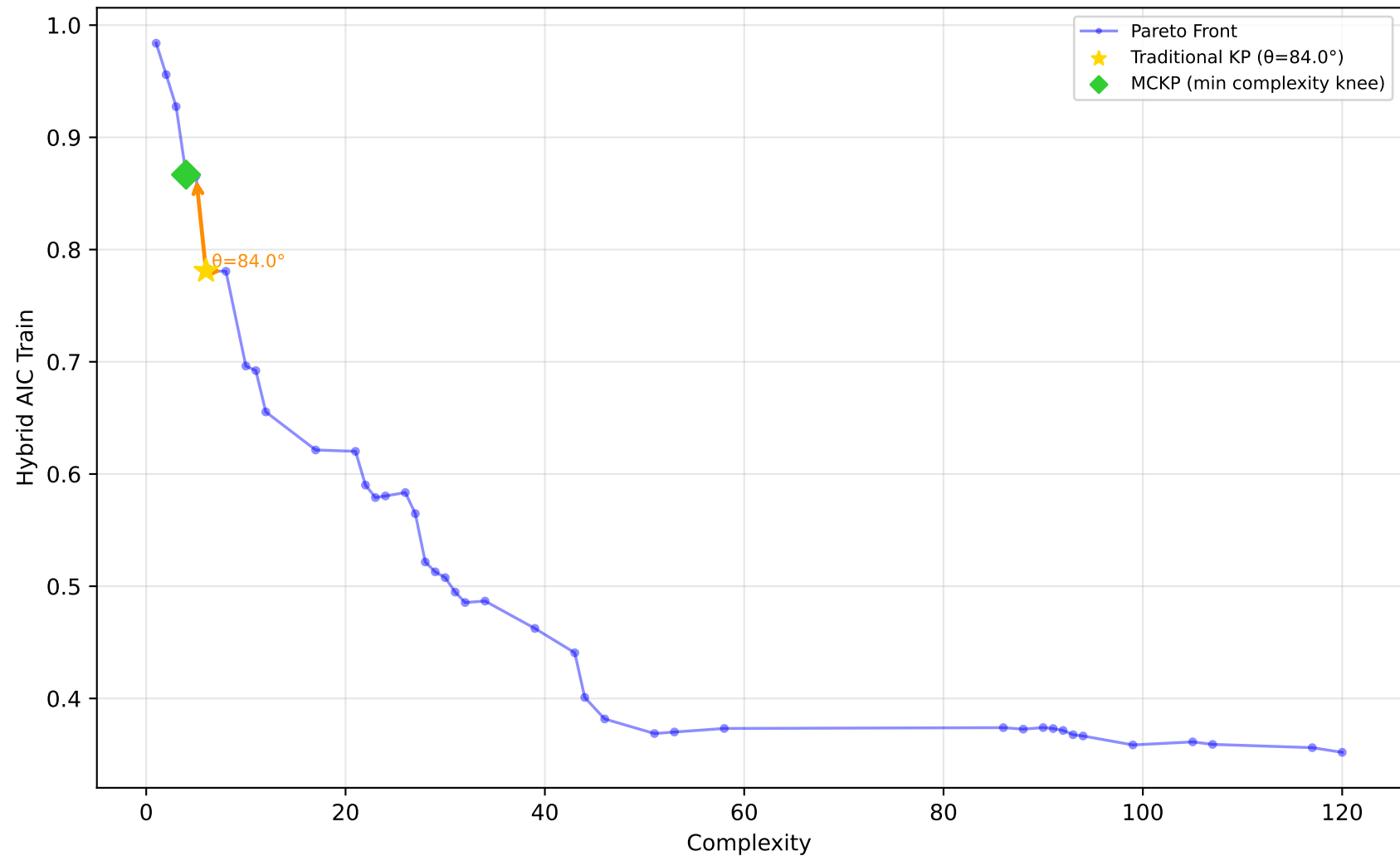
584_fri_c4_500_25 - Run 25 - MVP - Hybrid AIC Train \lambda_1=0.00, \lambda_2=0.00, \lambda_3=0.00 | Difficulty: 1.00 | Method: hmr
