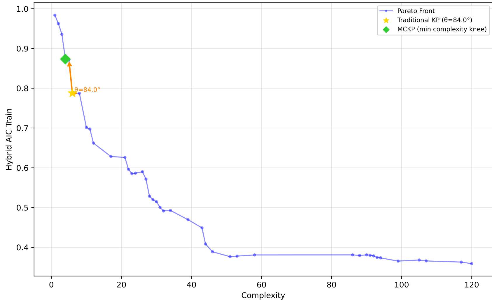
584_fri_c4_500_25 - Run 25 - MVP - Hybrid AIC Train \lambda_1=0.10, \lambda_2=0.00, \lambda_3=0.00 | Difficulty: 1.00 | Method: hmr
