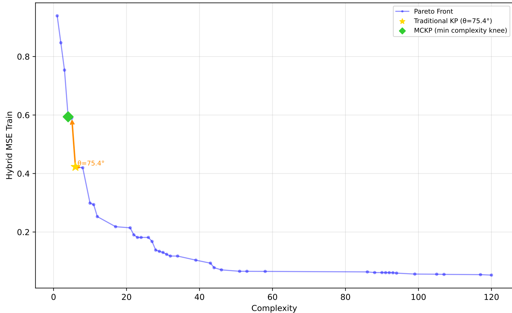
584_fri_c4_500_25 - Run 25 - MVP - Hybrid MSE Train \lambda_1=0.00, \lambda_2=0.00, \lambda_3=0.00 | Difficulty: 1.00 | Method: hmr
