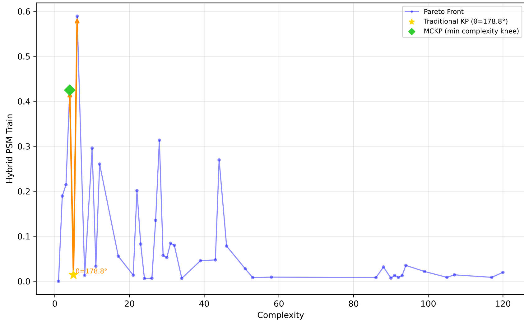
584_fri_c4_500_25 - Run 25 - MVP - Hybrid PSM Train \lambda_1=0.10, \bar{\lambda}_2=0.00, \bar{\lambda}_3=0.00 | Difficulty: 1.00 | Method: hmr
