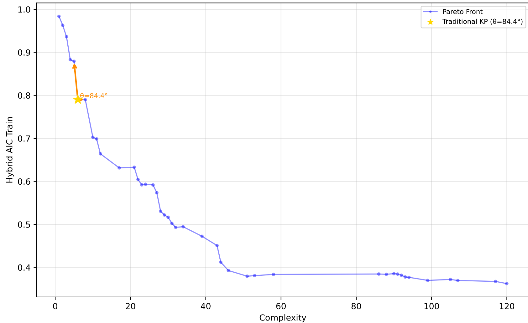
584_fri_c4_500_25 - Run 25 - SVP - Hybrid AIC Train \lambda_1=0.10 , \lambda_2=0.40 , \lambda_3=0.00 | Difficulty: 1.00 | Method: hmr
