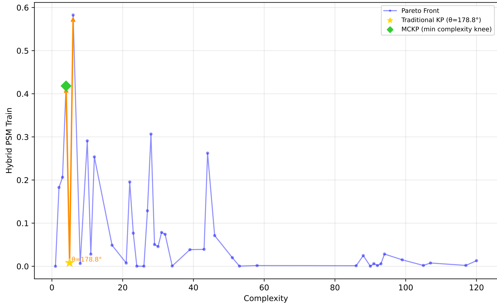
584_fri_c4_500_25 - Run 25 - SVP - Hybrid PSM Train \lambda_1=0.00, \lambda_2=0.00, \lambda_3=0.00 | Difficulty: 1.00 | Method: hmr
