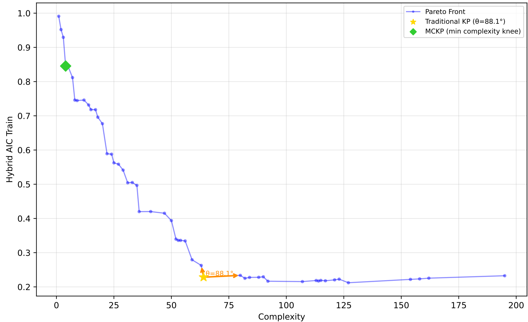
584_fri_c4_500_25 - Run 26 - MVP - Hybrid AIC Train \lambda_1=0.00, \lambda_2=0.00, \lambda_3=0.00 | Difficulty: 1.00 | Method: hmr
