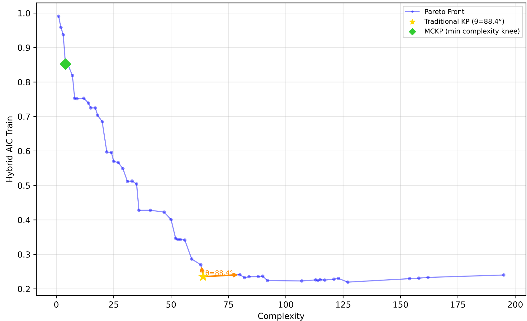
584_fri_c4_500_25 - Run 26 - MVP - Hybrid AIC Train \lambda_1=0.10, \lambda_2=0.00, \lambda_3=0.00 | Difficulty: 1.00 | Method: hmr
