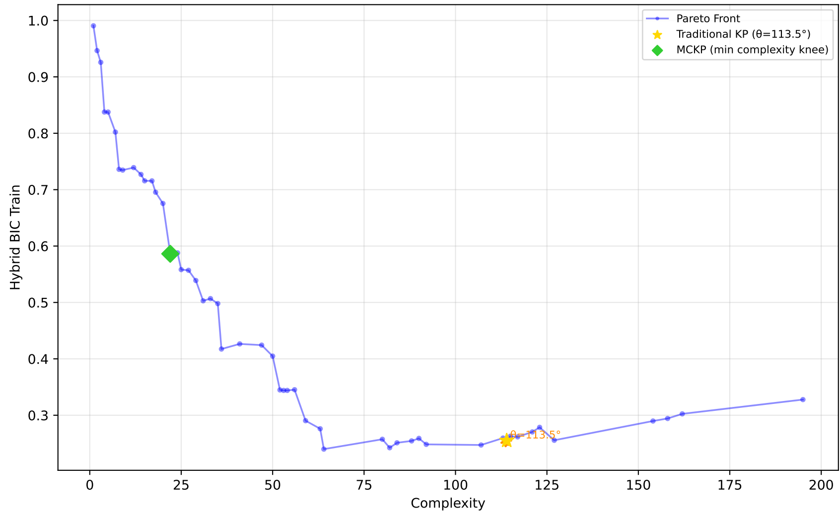
584_fri_c4_500_25 - Run 26 - MVP - Hybrid BIC Train \lambda_1=0.00, \lambda_2=0.00, \lambda_3=0.00 | Difficulty: 1.00 | Method: hmr
