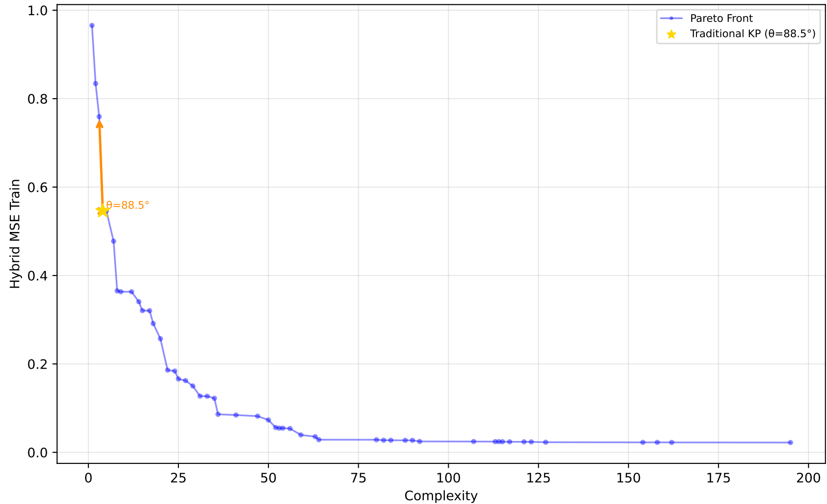
584_fri_c4_500_25 - Run 26 - MVP - Hybrid MSE Train \lambda_1=0.00, \bar{\lambda}_2=0.00, \bar{\lambda}_3=0.00 | Difficulty: 1.00 | Method: hmr
