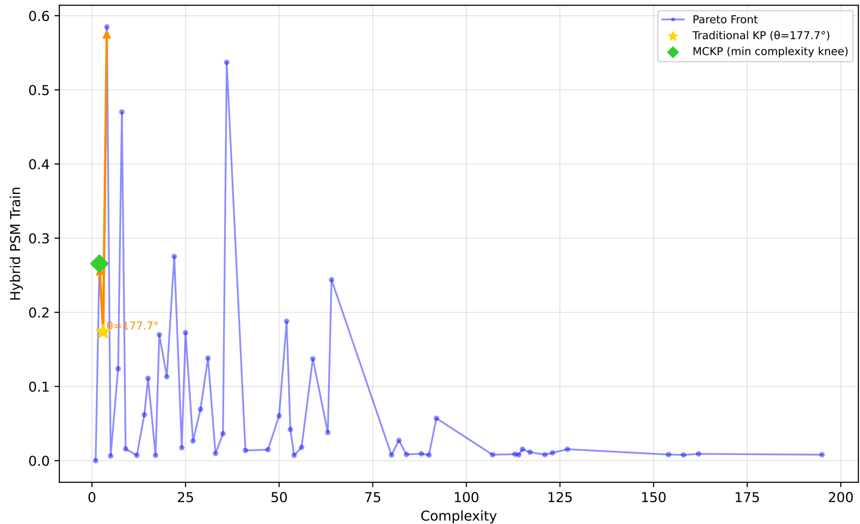
584_fri_c4_500_25 - Run 26 - MVP - Hybrid PSM Train \lambda_1=0.10, \bar{\lambda}_2=0.00, \bar{\lambda}_3=0.00 | Difficulty: 1.00 | Method: hmr
