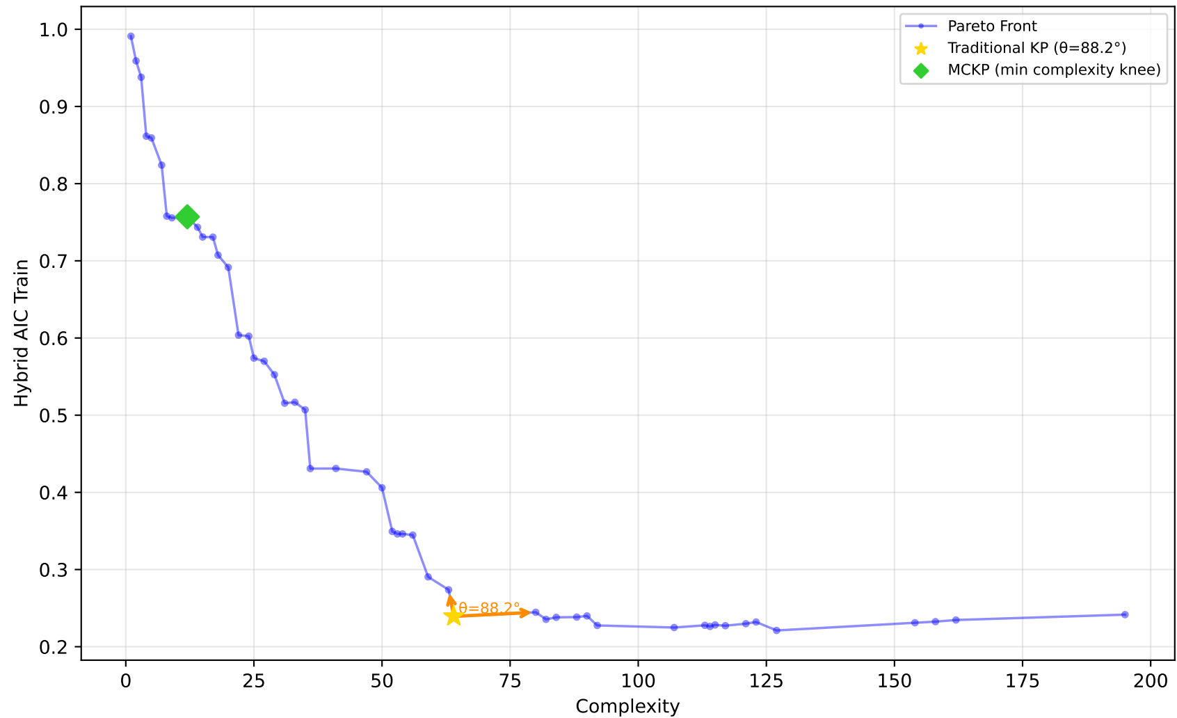
584_fri_c4_500_25 - Run 26 - SVP - Hybrid AIC Train \lambda_1=0.10, \lambda_2=0.40, \lambda_3=0.00 | Difficulty: 1.00 | Method: hmr
