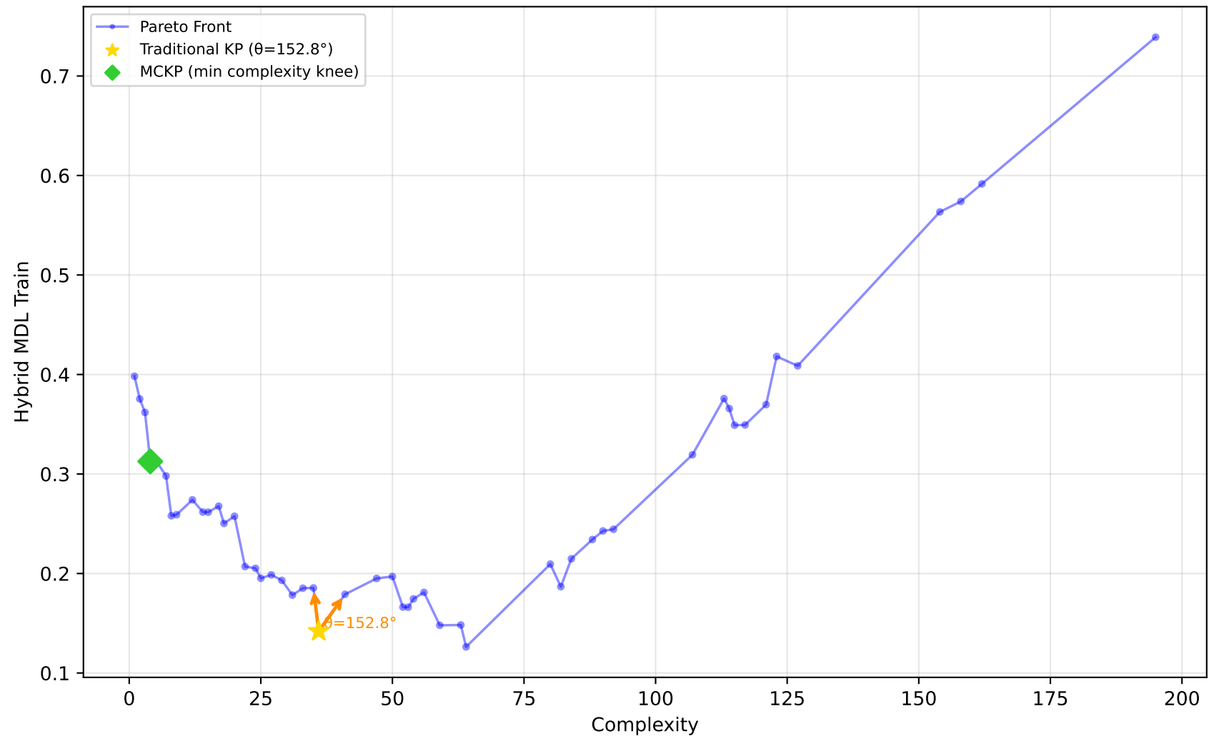
584_fri_c4_500_25 - Run 26 - SVP - Hybrid MDL Train \lambda_1=0.00, \lambda_2=0.00, \lambda_3=0.00 | Difficulty: 1.00 | Method: hmr
